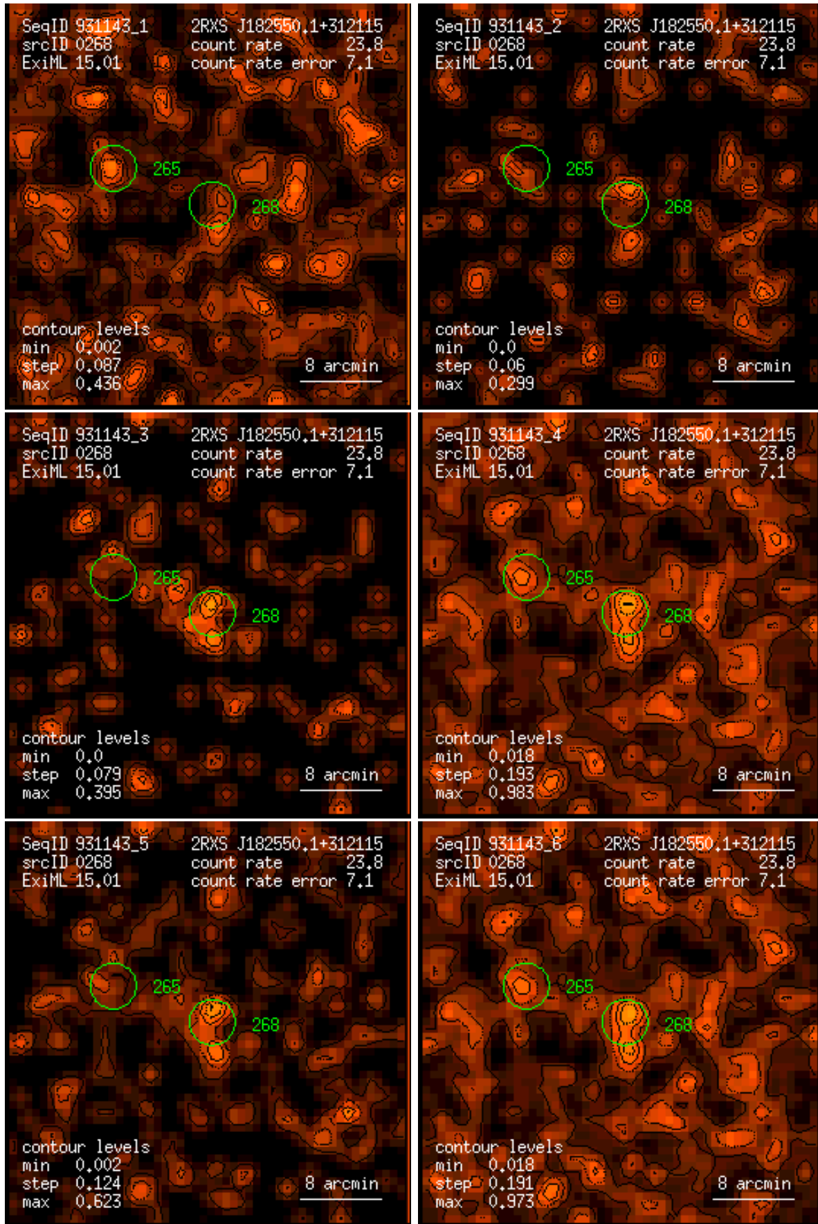
Figure 268: RASS 931143: detection 0268: band rate images, Gaussian filter: (1) PSPC channels 11 – 41, (2) 52 – 90, (3) 91 – 201, (4) 11 – 235, (5) 52 – 201, (6) 11 – 201. Broad band rates in counts/ks. Band rate contour levels in counts/ks/arcmin 2 .
