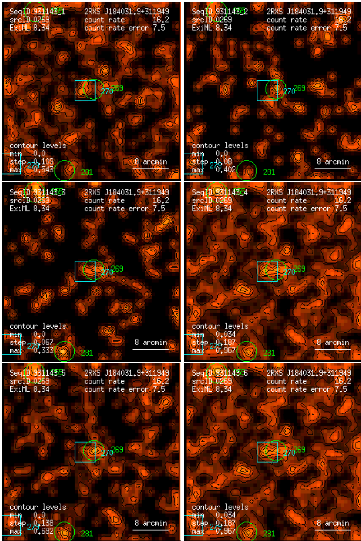
Figure 269: RASS 931143: detection 0269: band rate images, Gaussian filter: (1) PSPC channels 11 – 41, (2) 52 – 90, (3) 91 – 201, (4) 11 – 235, (5) 52 – 201, (6) 11 – 201. Broad band rates in counts/ks. Band rate contour levels in counts/ks/arcmin 2 .
