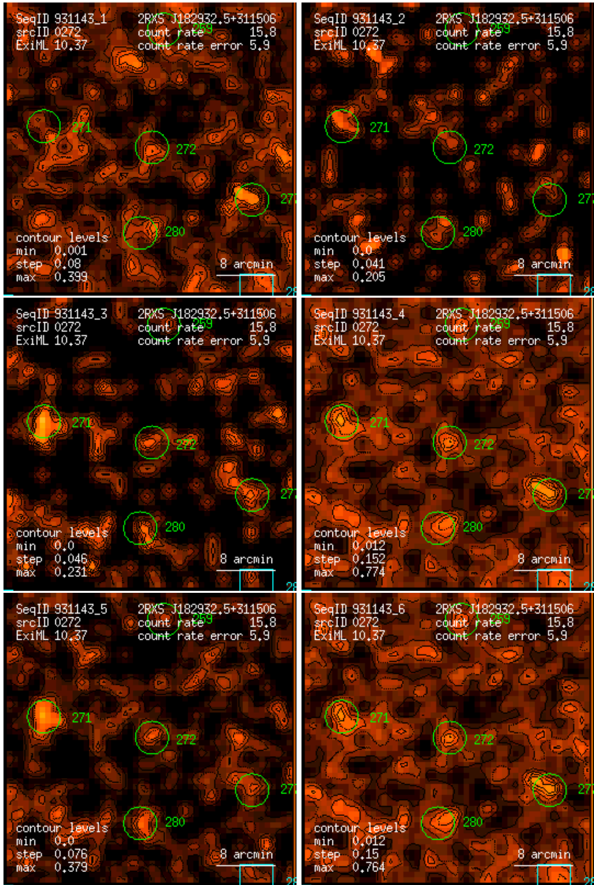
Figure 272: RASS 931143: detection 0272: band rate images, Gaussian filter: (1) PSPC channels 11 – 41, (2) 52 – 90, (3) 91 – 201, (4) 11 – 235, (5) 52 – 201, (6) 11 – 201. Broad band rates in counts/ks. Band rate contour levels in counts/ks/arcmin 2 .
