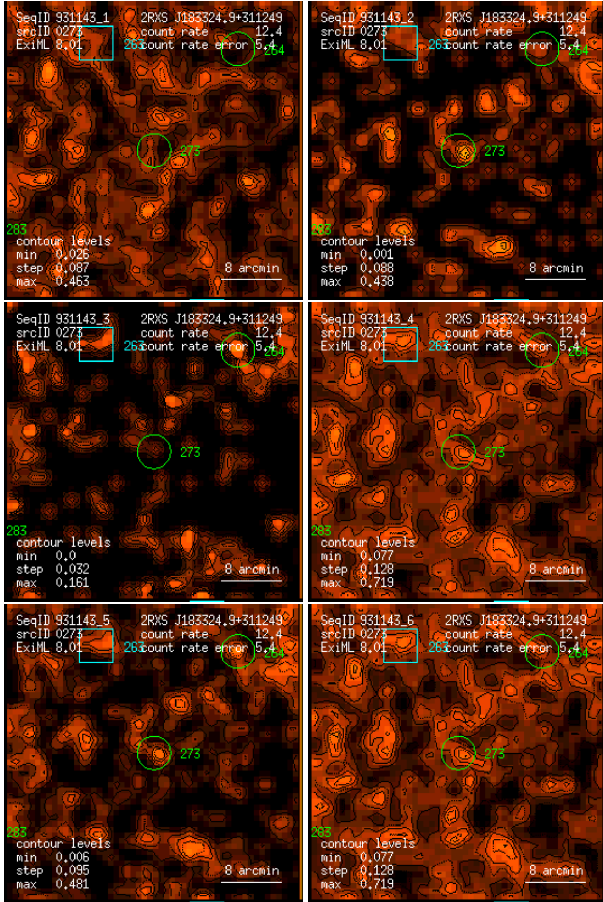
Figure 273: RASS 931143: detection 0273: band rate images, Gaussian filter: (1) PSPC channels 11 – 41, (2) 52 – 90, (3) 91 – 201, (4) 11 – 235, (5) 52 – 201, (6) 11 – 201. Broad band rates in counts/ks. Band rate contour levels in counts/ks/arcmin 2 .
