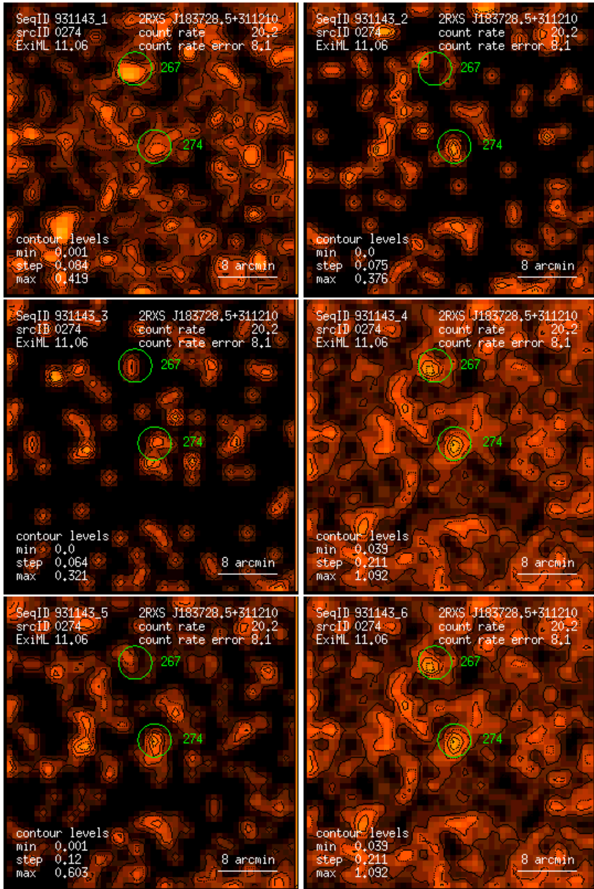
Figure 274: RASS 931143: detection 0274: band rate images, Gaussian filter: (1) PSPC channels 11 – 41, (2) 52 – 90, (3) 91 – 201, (4) 11 – 235, (5) 52 – 201, (6) 11 – 201. Broad band rates in counts/ks. Band rate contour levels in counts/ks/arcmin 2 .
