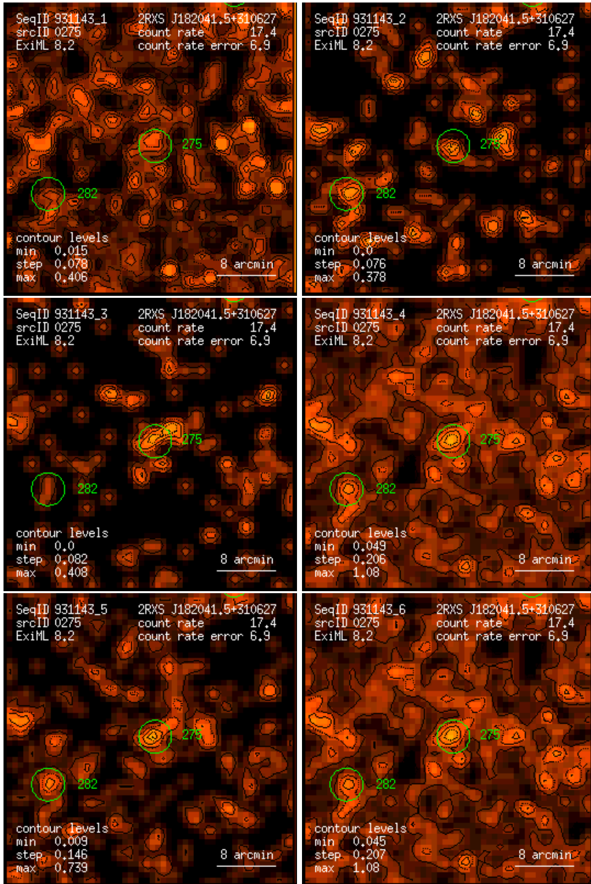
Figure 275: RASS 931143: detection 0275: band rate images, Gaussian filter: (1) PSPC channels 11 – 41, (2) 52 – 90, (3) 91 – 201, (4) 11 – 235, (5) 52 – 201, (6) 11 – 201. Broad band rates in counts/ks. Band rate contour levels in counts/ks/arcmin 2 .
