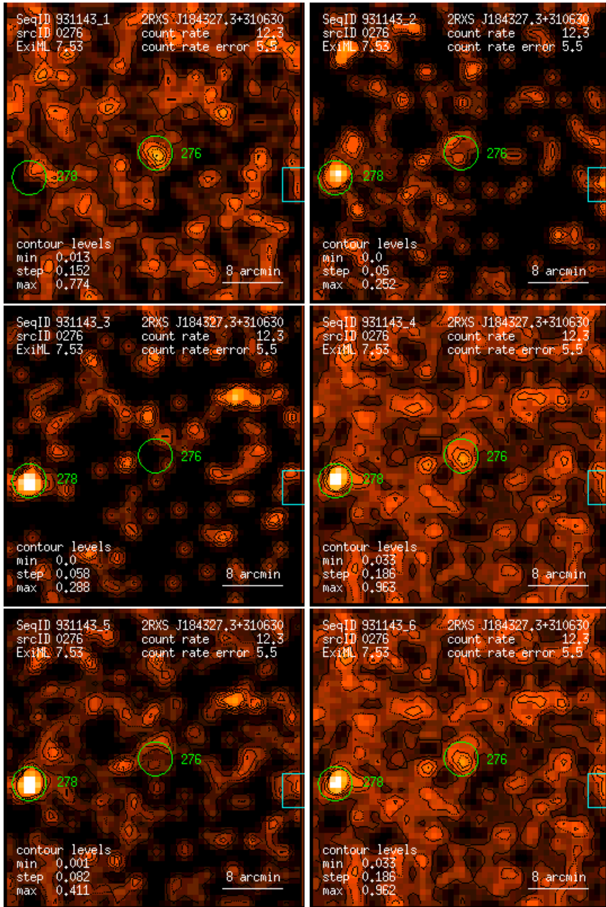
Figure 276: RASS 931143: detection 0276: band rate images, Gaussian filter: (1) PSPC channels 11 – 41, (2) 52 – 90, (3) 91 – 201, (4) 11 – 235, (5) 52 – 201, (6) 11 – 201. Broad band rates in counts/ks. Band rate contour levels in counts/ks/arcmin 2 .
