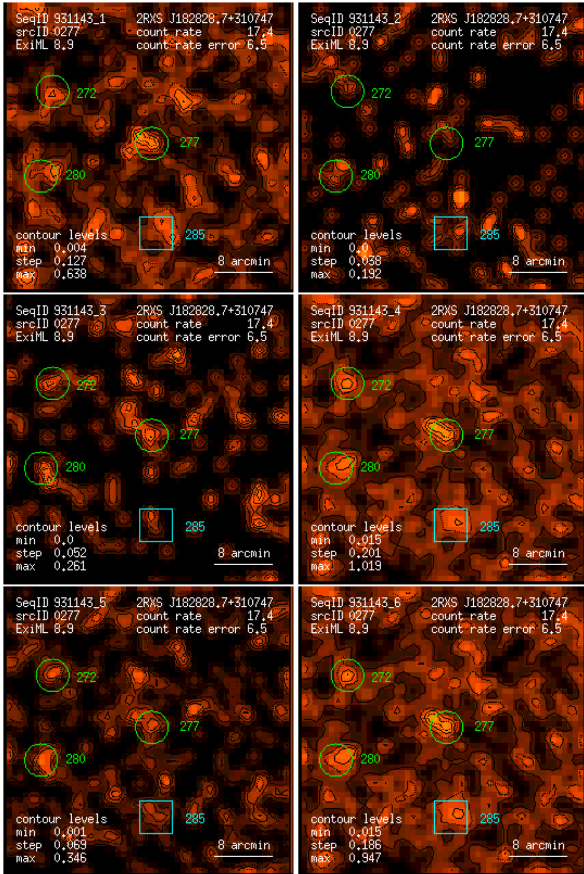
Figure 277: RASS 931143: detection 0277: band rate images, Gaussian filter: (1) PSPC channels 11 – 41, (2) 52 – 90, (3) 91 – 201, (4) 11 – 235, (5) 52 – 201, (6) 11 – 201. Broad band rates in counts/ks. Band rate contour levels in counts/ks/arcmin 2 .
