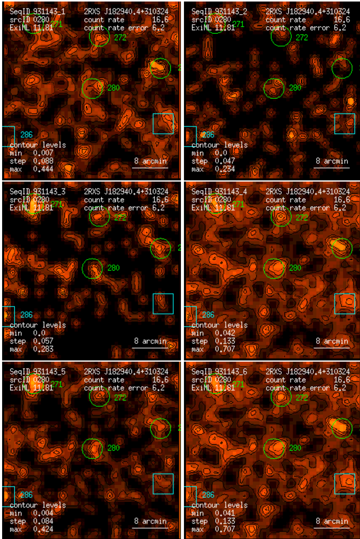
Figure 280: RASS 931143: detection 0280: band rate images, Gaussian filter: (1) PSPC channels 11 – 41, (2) 52 – 90, (3) 91 – 201, (4) 11 – 235, (5) 52 – 201, (6) 11 – 201. Broad band rates in counts/ks. Band rate contour levels in counts/ks/arcmin 2 .
