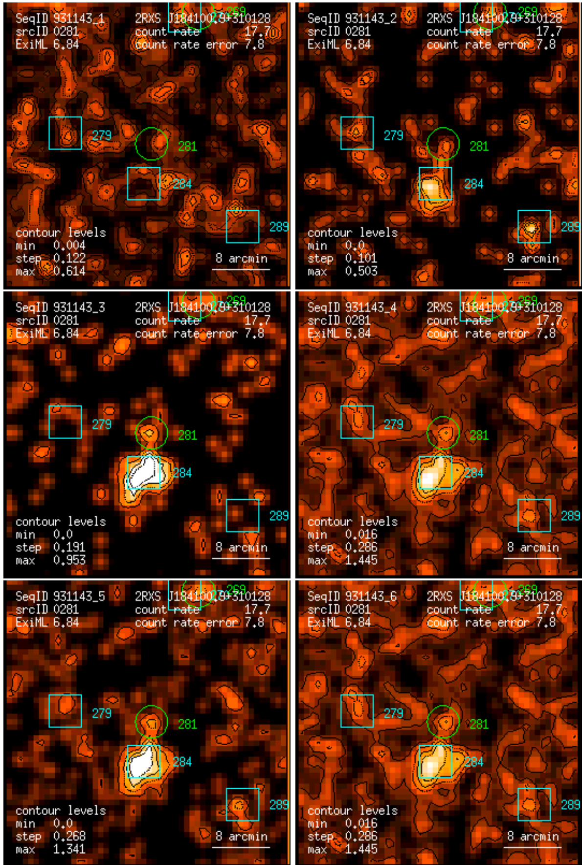
Figure 281: RASS 931143: detection 0281: band rate images, Gaussian filter: (1) PSPC channels 11 – 41, (2) 52 – 90, (3) 91 – 201, (4) 11 – 235, (5) 52 – 201, (6) 11 – 201. Broad band rates in counts/ks. Band rate contour levels in counts/ks/arcmin 2 .
