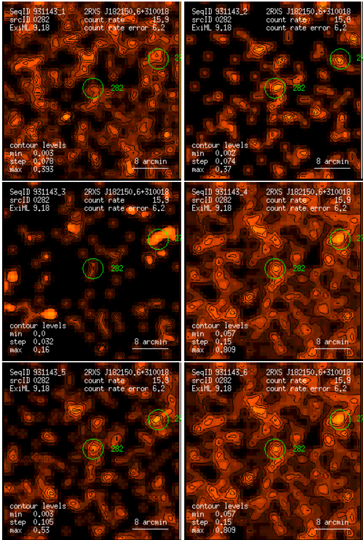
Figure 282: RASS 931143: detection 0282: band rate images, Gaussian filter: (1) PSPC channels 11 – 41, (2) 52 – 90, (3) 91 – 201, (4) 11 – 235, (5) 52 – 201, (6) 11 – 201. Broad band rates in counts/ks. Band rate contour levels in counts/ks/arcmin 2 .
