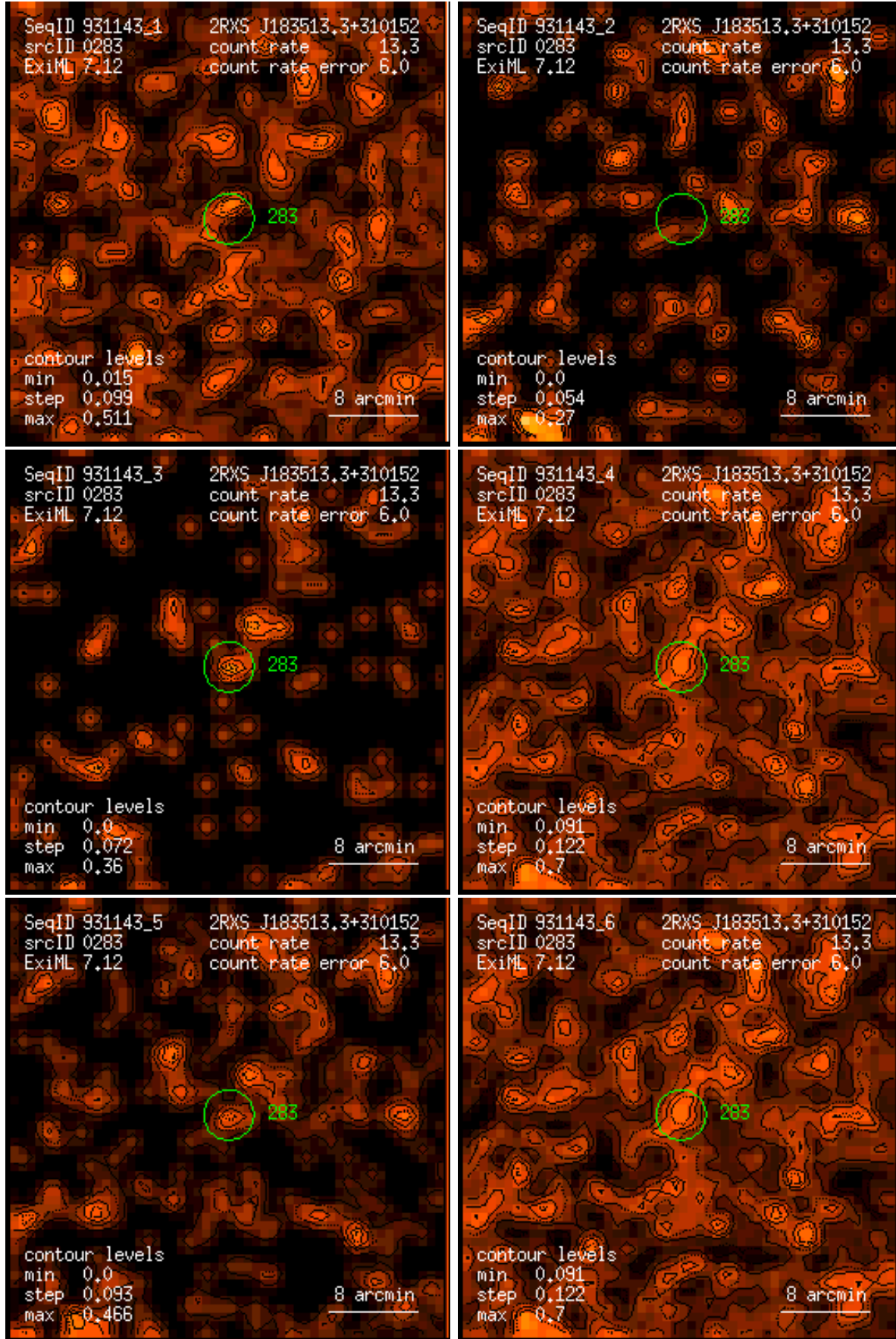
Figure 283: RASS 931143: detection 0283: band rate images, Gaussian filter: (1) PSPC channels 11 – 41, (2) 52 – 90, (3) 91 – 201, (4) 11 – 235, (5) 52 – 201, (6) 11 – 201. Broad band rates in counts/ks. Band rate contour levels in counts/ks/arcmin 2 .
