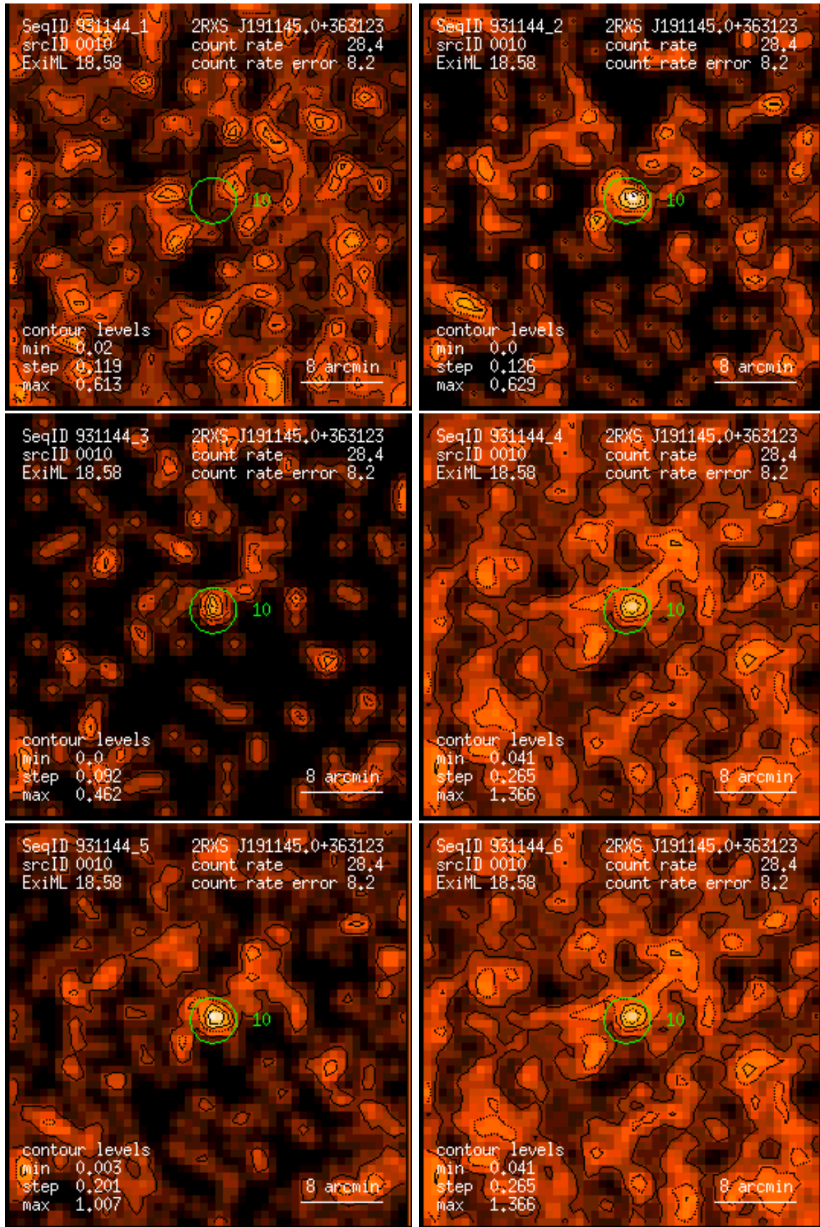
Figure 10: RASS 931144: detection 0010: band rate images, Gaussian filter: (1) PSPC channels 11 – 41, (2) 52 – 90, (3) 91 – 201, (4) 11 – 235, (5) 52 – 201, (6) 11 – 201. Broad band rates in counts/ks. Band rate contour levels in counts/ks/arcmin 2 .
