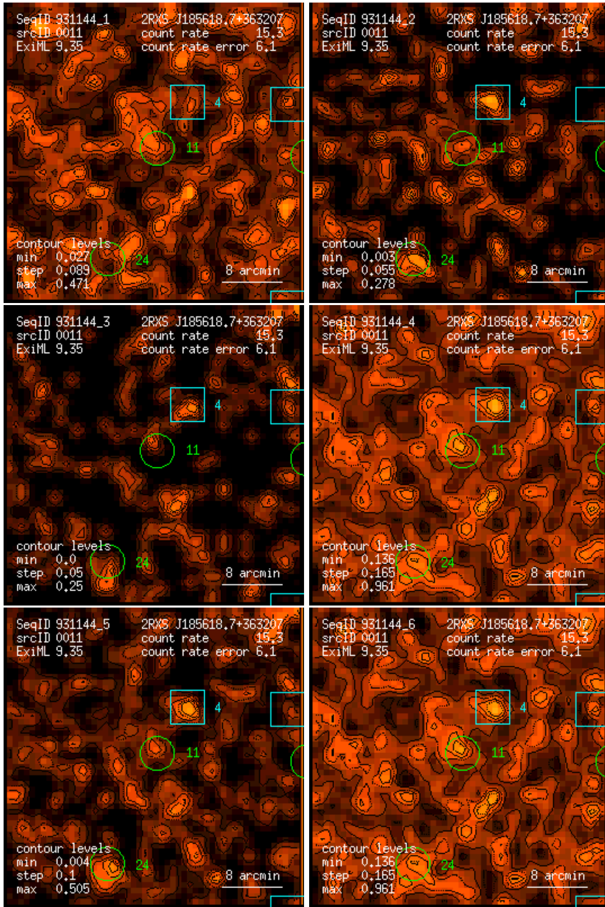
Figure 11: RASS 931144: detection 0011: band rate images, Gaussian filter: (1) PSPC channels 11 – 41, (2) 52 – 90, (3) 91 – 201, (4) 11 – 235, (5) 52 – 201, (6) 11 – 201. Broad band rates in counts/ks. Band rate contour levels in counts/ks/arcmin 2 .
