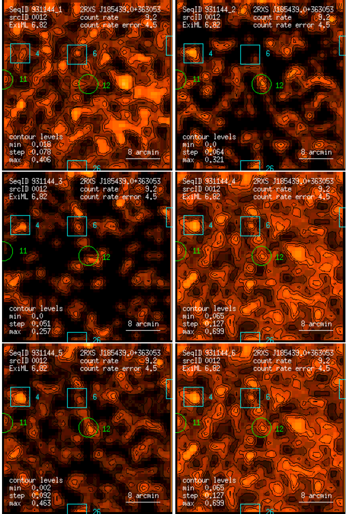
Figure 12: RASS 931144: detection 0012: band rate images, Gaussian filter: (1) PSPC channels 11 – 41, (2) 52 – 90, (3) 91 – 201, (4) 11 – 235, (5) 52 – 201, (6) 11 – 201. Broad band rates in counts/ks. Band rate contour levels in counts/ks/arcmin 2 .
