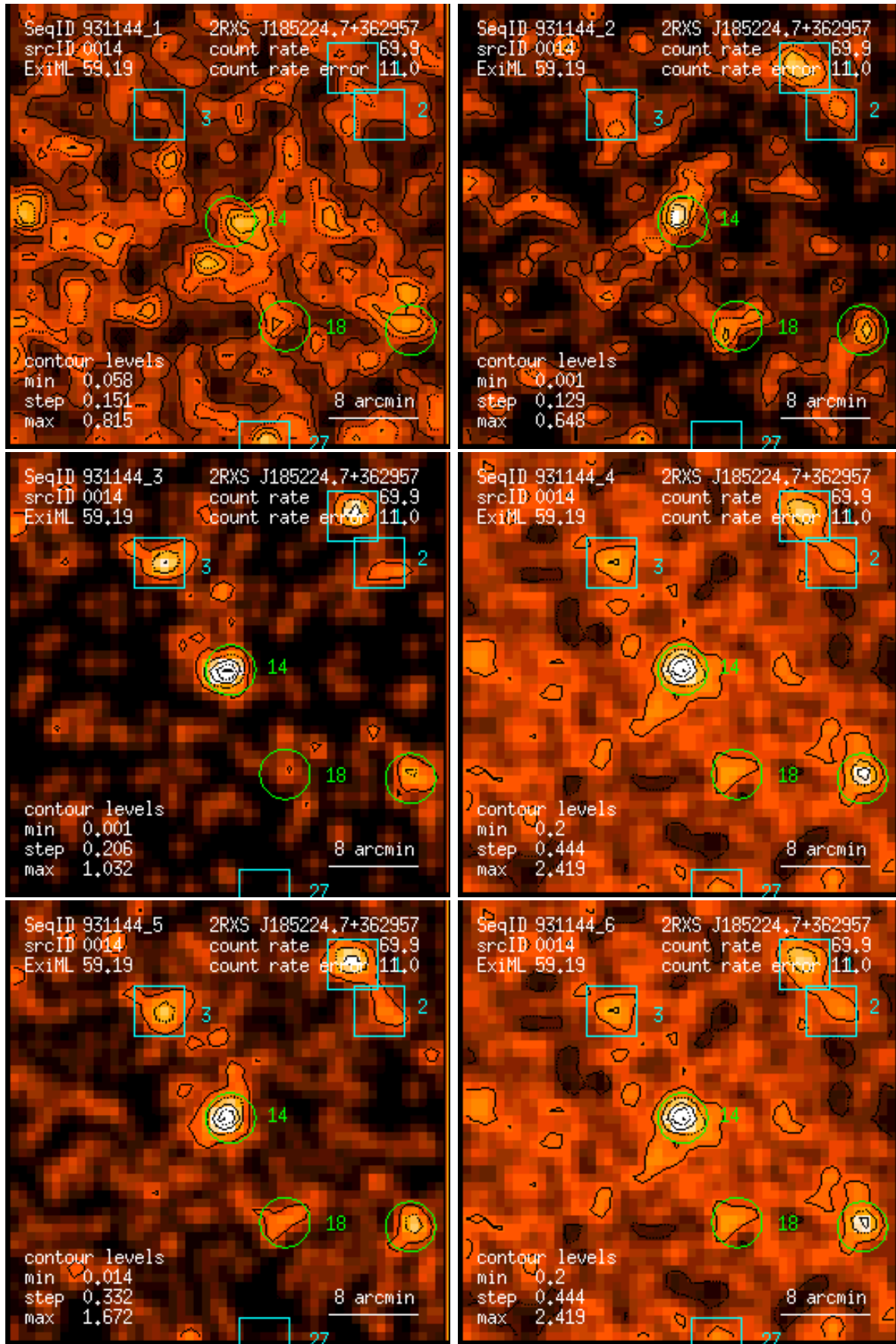
Figure 14: RASS 931144: detection 0014: band rate images, Gaussian filter: (1) PSPC channels 11 – 41, (2) 52 – 90, (3) 91 – 201, (4) 11 – 235, (5) 52 – 201, (6) 11 – 201. Broad band rates in counts/ks. Band rate contour levels in counts/ks/arcmin 2 .
