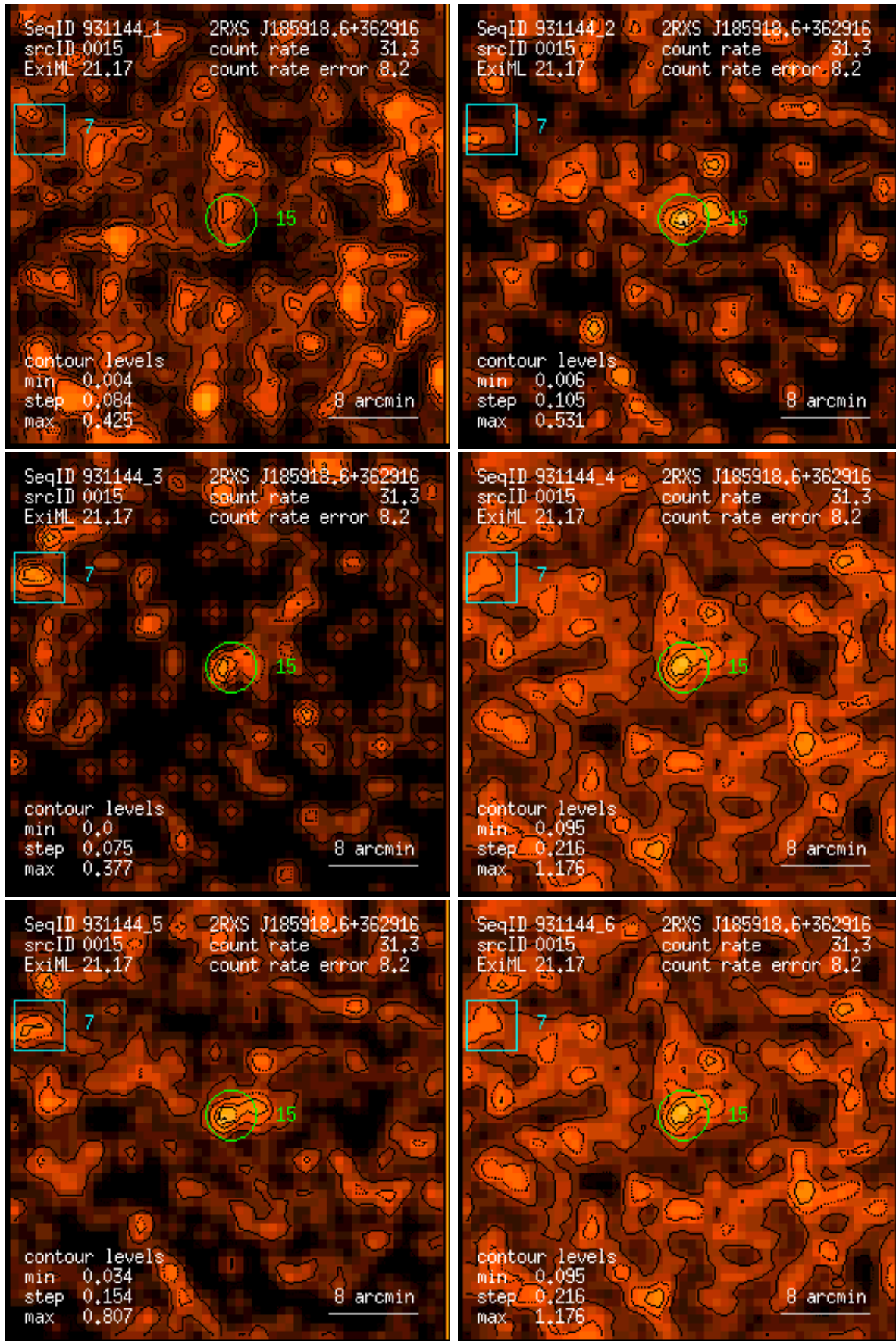
Figure 15: RASS 931144: detection 0015: band rate images, Gaussian filter: (1) PSPC channels 11 – 41, (2) 52 – 90, (3) 91 – 201, (4) 11 – 235, (5) 52 – 201, (6) 11 – 201. Broad band rates in counts/ks. Band rate contour levels in counts/ks/arcmin 2 .
