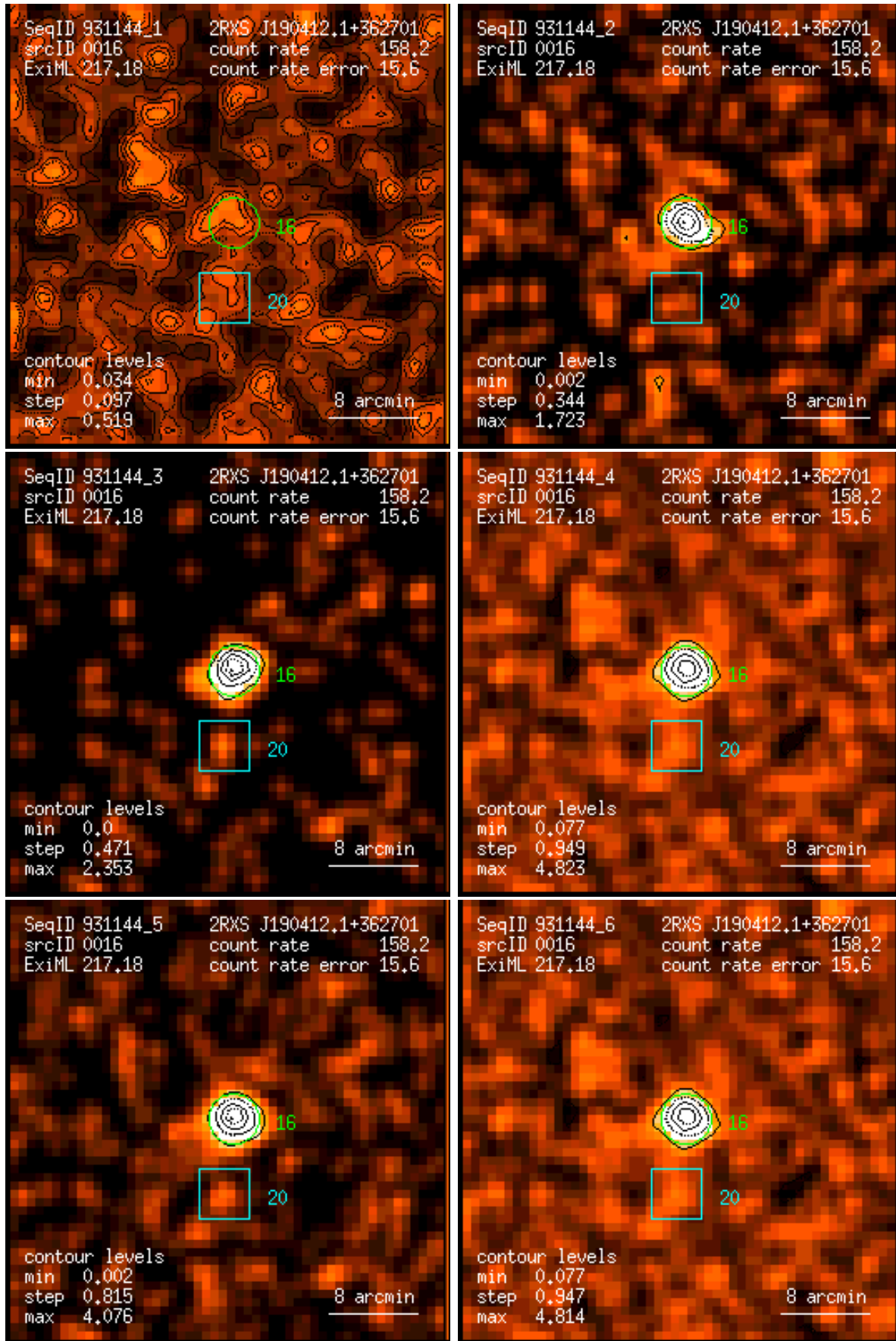
Figure 16: RASS 931144: detection 0016: band rate images, Gaussian filter: (1) PSPC channels 11 – 41, (2) 52 – 90, (3) 91 – 201, (4) 11 – 235, (5) 52 – 201, (6) 11 – 201. Broad band rates in counts/ks. Band rate contour levels in counts/ks/arcmin 2 .
