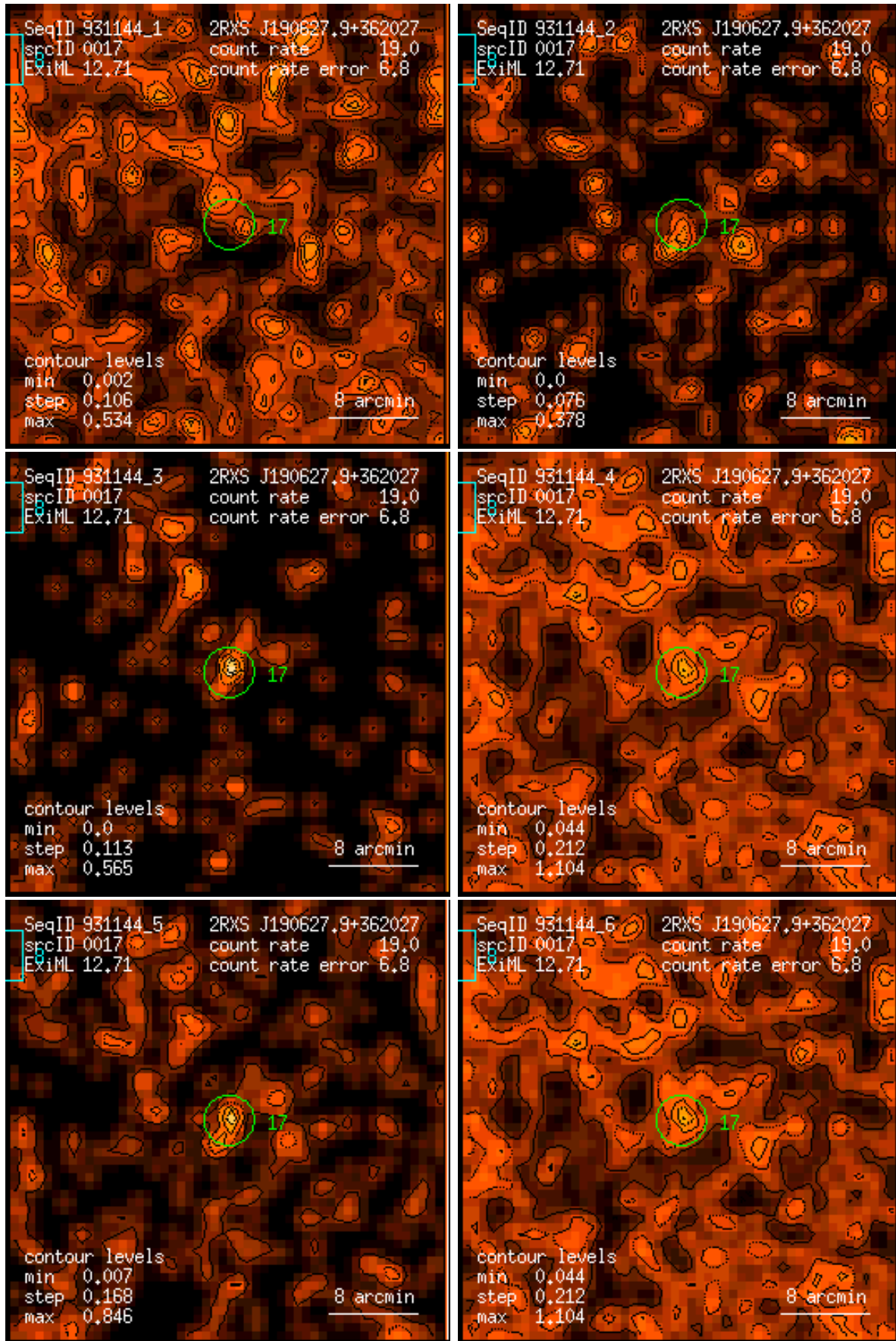
Figure 17: RASS 931144: detection 0017: band rate images, Gaussian filter: (1) PSPC channels 11 – 41, (2) 52 – 90, (3) 91 – 201, (4) 11 – 235, (5) 52 – 201, (6) 11 – 201. Broad band rates in counts/ks. Band rate contour levels in counts/ks/arcmin 2 .
