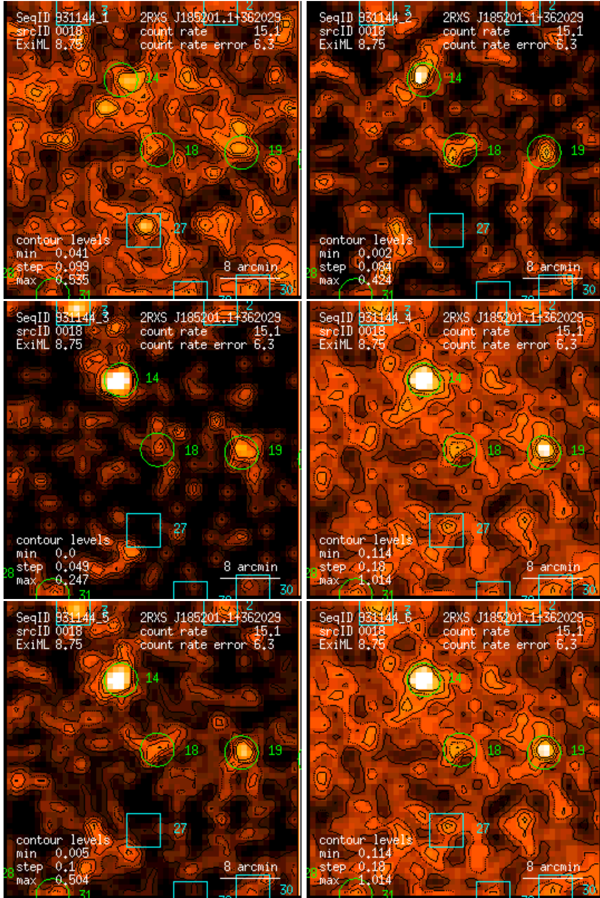
Figure 18: RASS 931144: detection 0018: band rate images, Gaussian filter: (1) PSPC channels 11 – 41, (2) 52 – 90, (3) 91 – 201, (4) 11 – 235, (5) 52 – 201, (6) 11 – 201. Broad band rates in counts/ks. Band rate contour levels in counts/ks/arcmin 2 .
