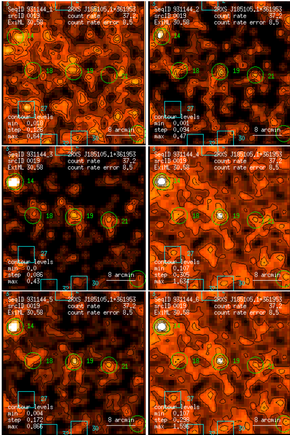
Figure 19: RASS 931144: detection 0019: band rate images, Gaussian filter: (1) PSPC channels 11 – 41, (2) 52 – 90, (3) 91 – 201, (4) 11 – 235, (5) 52 – 201, (6) 11 – 201. Broad band rates in counts/ks. Band rate contour levels in counts/ks/arcmin 2 .
