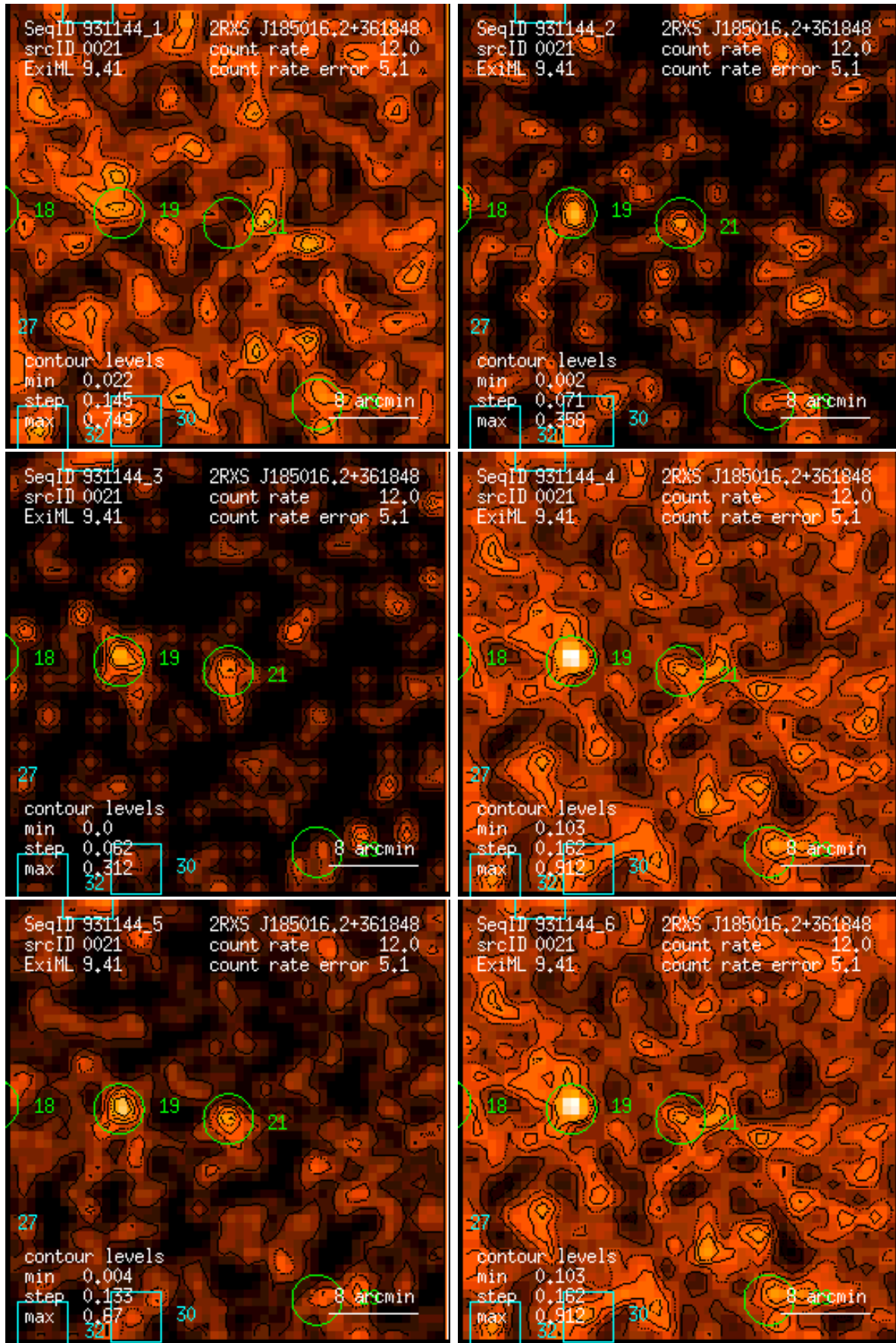
Figure 21: RASS 931144: detection 0021: band rate images, Gaussian filter: (1) PSPC channels 11 – 41, (2) 52 – 90, (3) 91 – 201, (4) 11 – 235, (5) 52 – 201, (6) 11 – 201. Broad band rates in counts/ks. Band rate contour levels in counts/ks/arcmin 2 .
