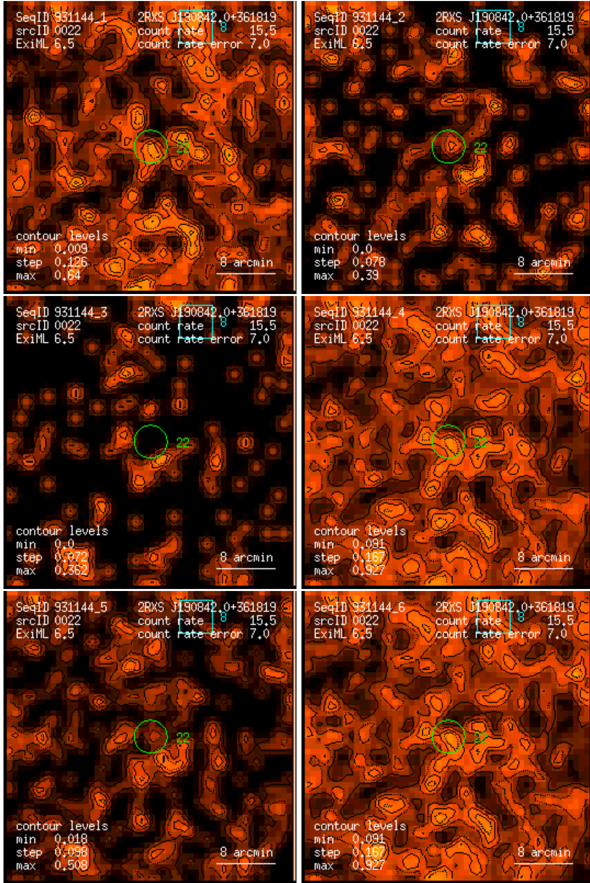
Figure 22: RASS 931144: detection 0022: band rate images, Gaussian filter: (1) PSPC channels 11 – 41, (2) 52 – 90, (3) 91 – 201, (4) 11 – 235, (5) 52 – 201, (6) 11 – 201. Broad band rates in counts/ks. Band rate contour levels in counts/ks/arcmin 2 .
