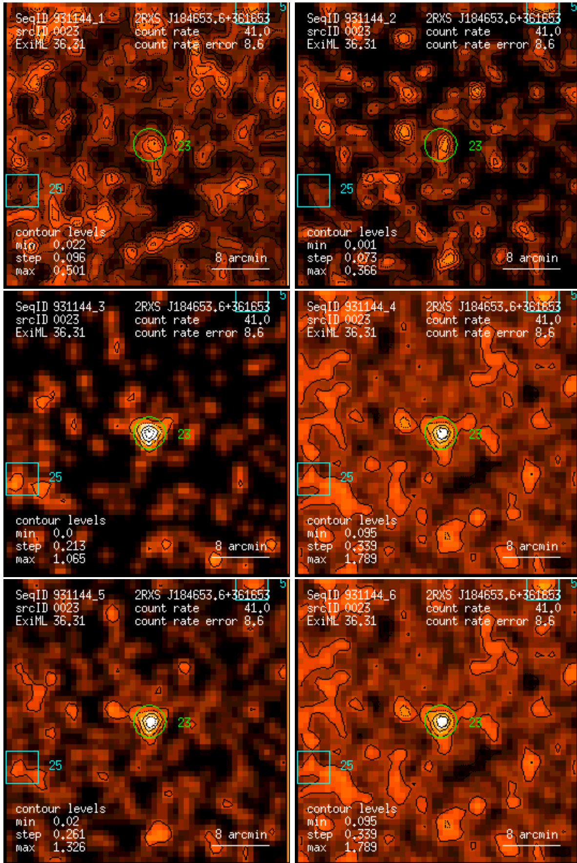
Figure 23: RASS 931144: detection 0023: band rate images, Gaussian filter: (1) PSPC channels 11 – 41, (2) 52 – 90, (3) 91 – 201, (4) 11 – 235, (5) 52 – 201, (6) 11 – 201. Broad band rates in counts/ks. Band rate contour levels in counts/ks/arcmin 2 .
