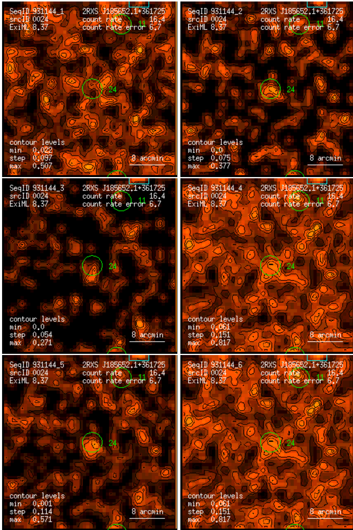
Figure 24: RASS 931144: detection 0024: band rate images, Gaussian filter: (1) PSPC channels 11 – 41, (2) 52 – 90, (3) 91 – 201, (4) 11 – 235, (5) 52 – 201, (6) 11 – 201. Broad band rates in counts/ks. Band rate contour levels in counts/ks/arcmin 2 .
