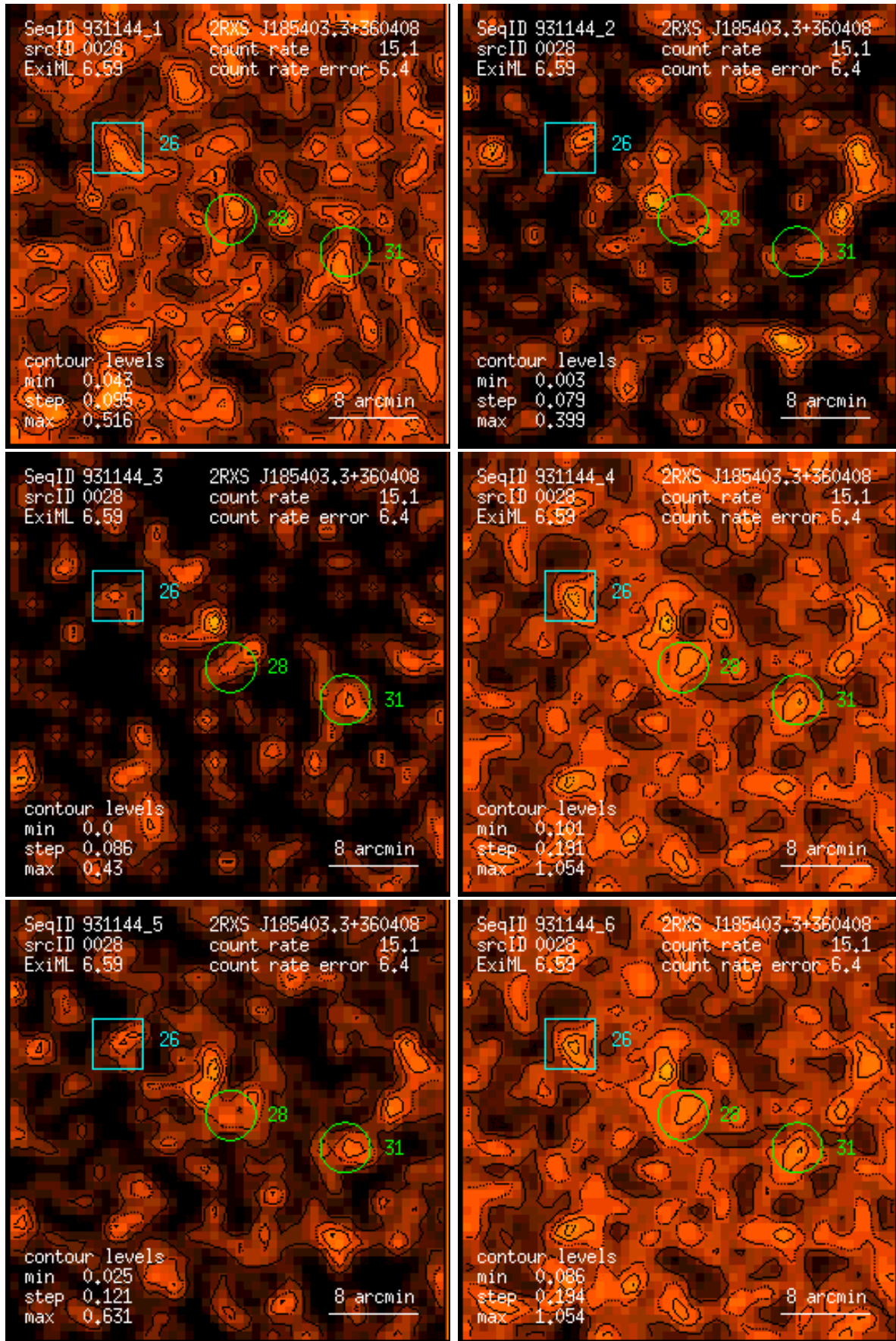
Figure 28: RASS 931144: detection 0028: band rate images, Gaussian filter: (1) PSPC channels 11 – 41, (2) 52 – 90, (3) 91 – 201, (4) 11 – 235, (5) 52 – 201, (6) 11 – 201. Broad band rates in counts/ks. Band rate contour levels in counts/ks/arcmin 2 .
