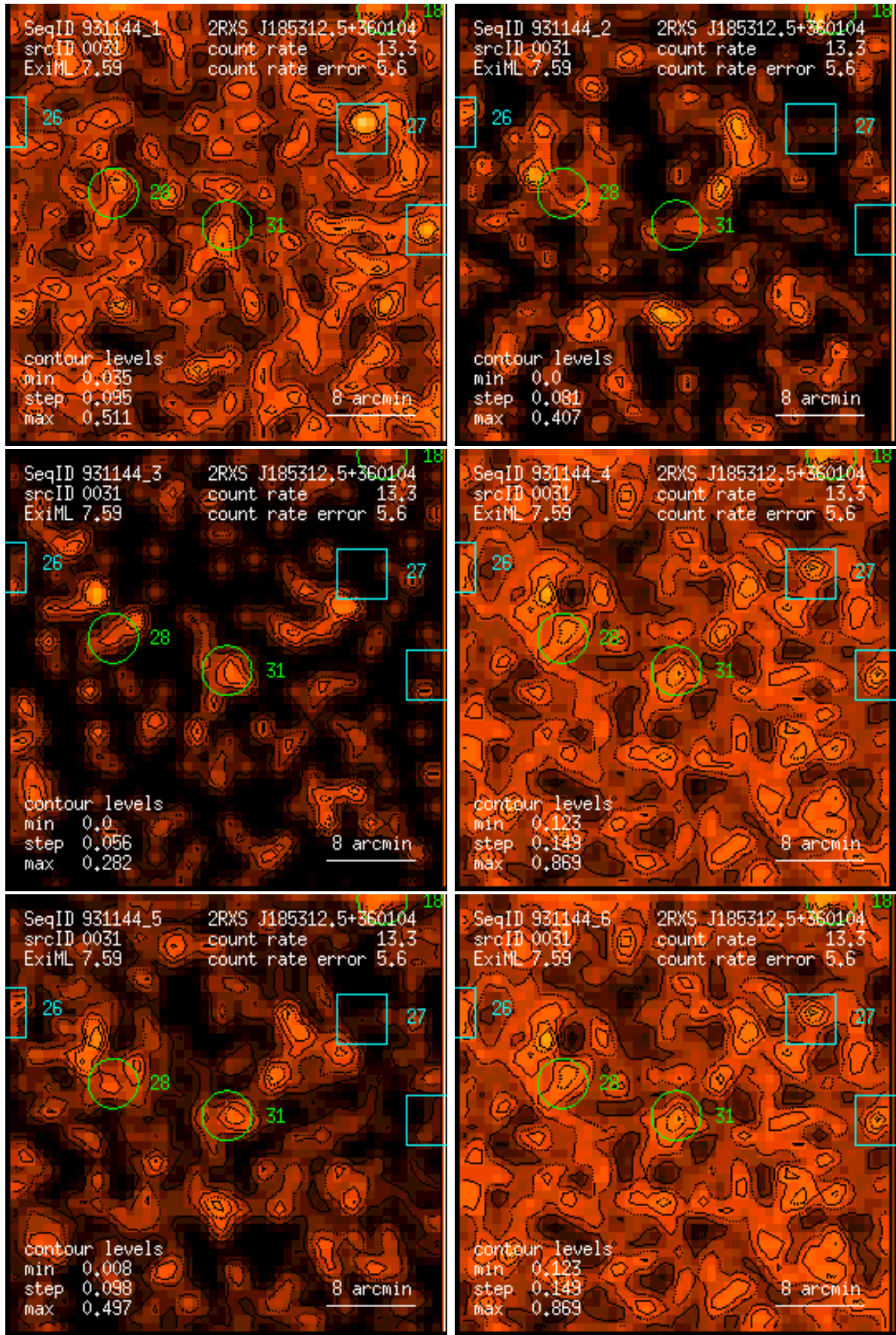
Figure 31: RASS 931144: detection 0031: band rate images, Gaussian filter: (1) PSPC channels 11 – 41, (2) 52 – 90, (3) 91 – 201, (4) 11 – 235, (5) 52 – 201, (6) 11 – 201. Broad band rates in counts/ks. Band rate contour levels in counts/ks/arcmin 2 .
