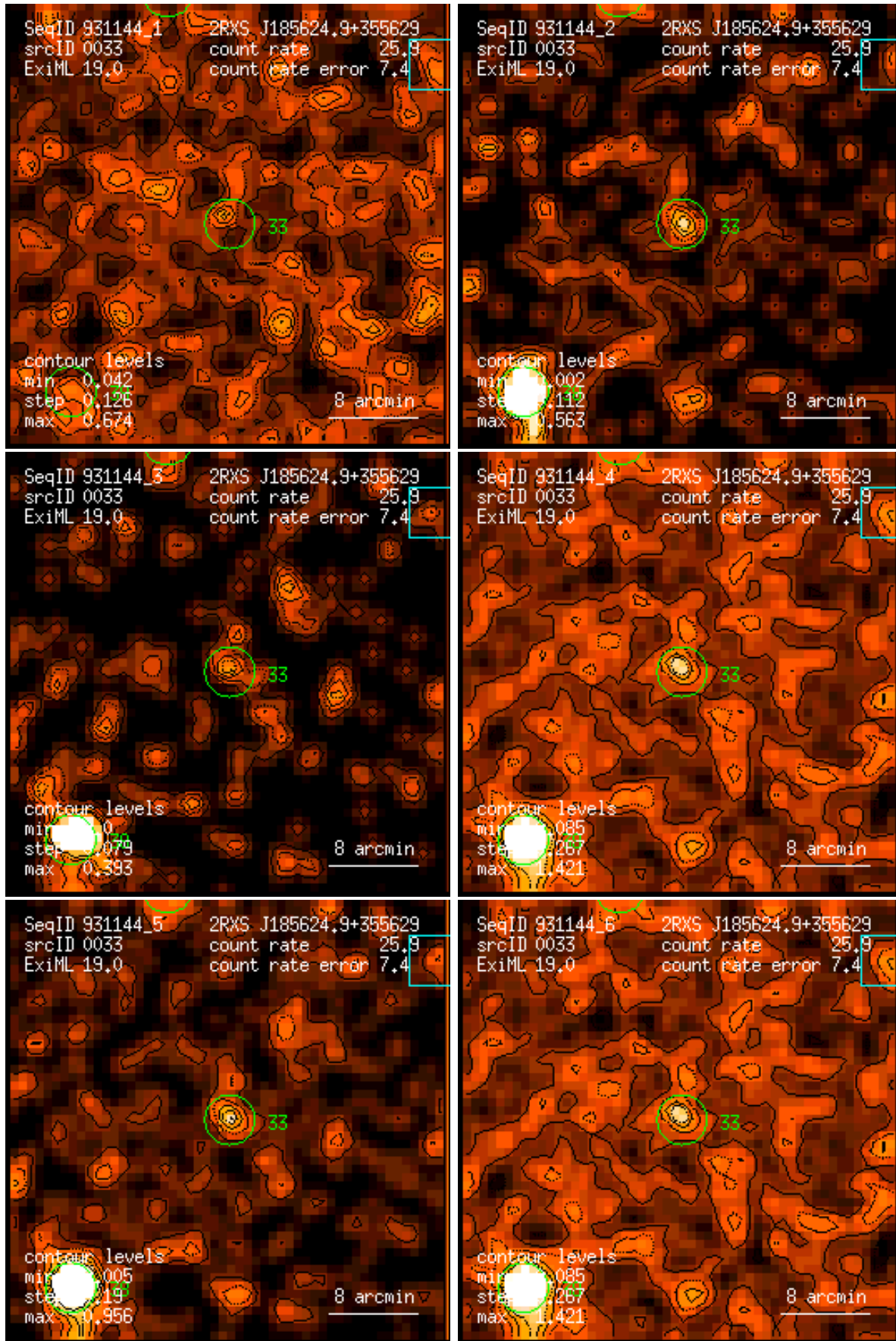
Figure 33: RASS 931144: detection 0033: band rate images, Gaussian filter: (1) PSPC channels 11 – 41, (2) 52 – 90, (3) 91 – 201, (4) 11 – 235, (5) 52 – 201, (6) 11 – 201. Broad band rates in counts/ks. Band rate contour levels in counts/ks/arcmin 2 .
