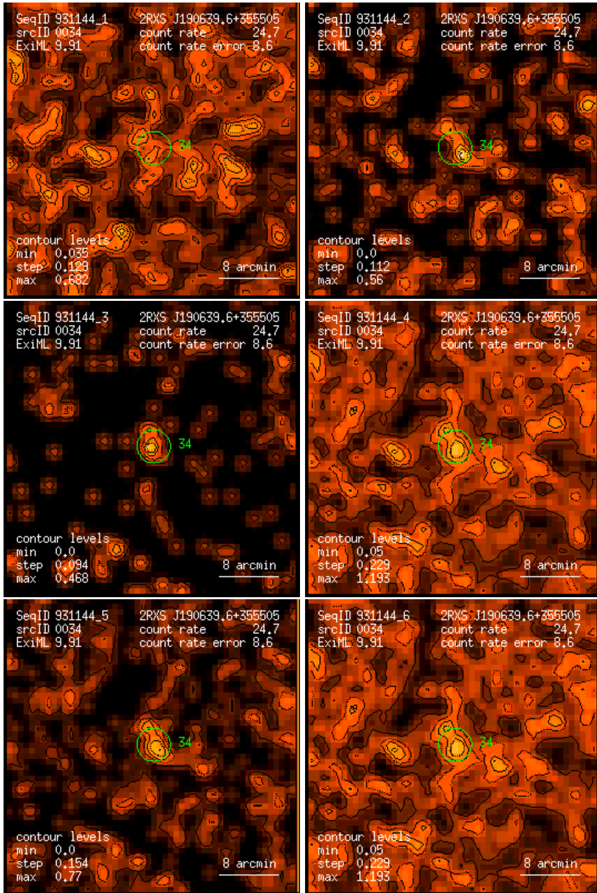
Figure 34: RASS 931144: detection 0034: band rate images, Gaussian filter: (1) PSPC channels 11 – 41, (2) 52 – 90, (3) 91 – 201, (4) 11 – 235, (5) 52 – 201, (6) 11 – 201. Broad band rates in counts/ks. Band rate contour levels in counts/ks/arcmin 2 .
