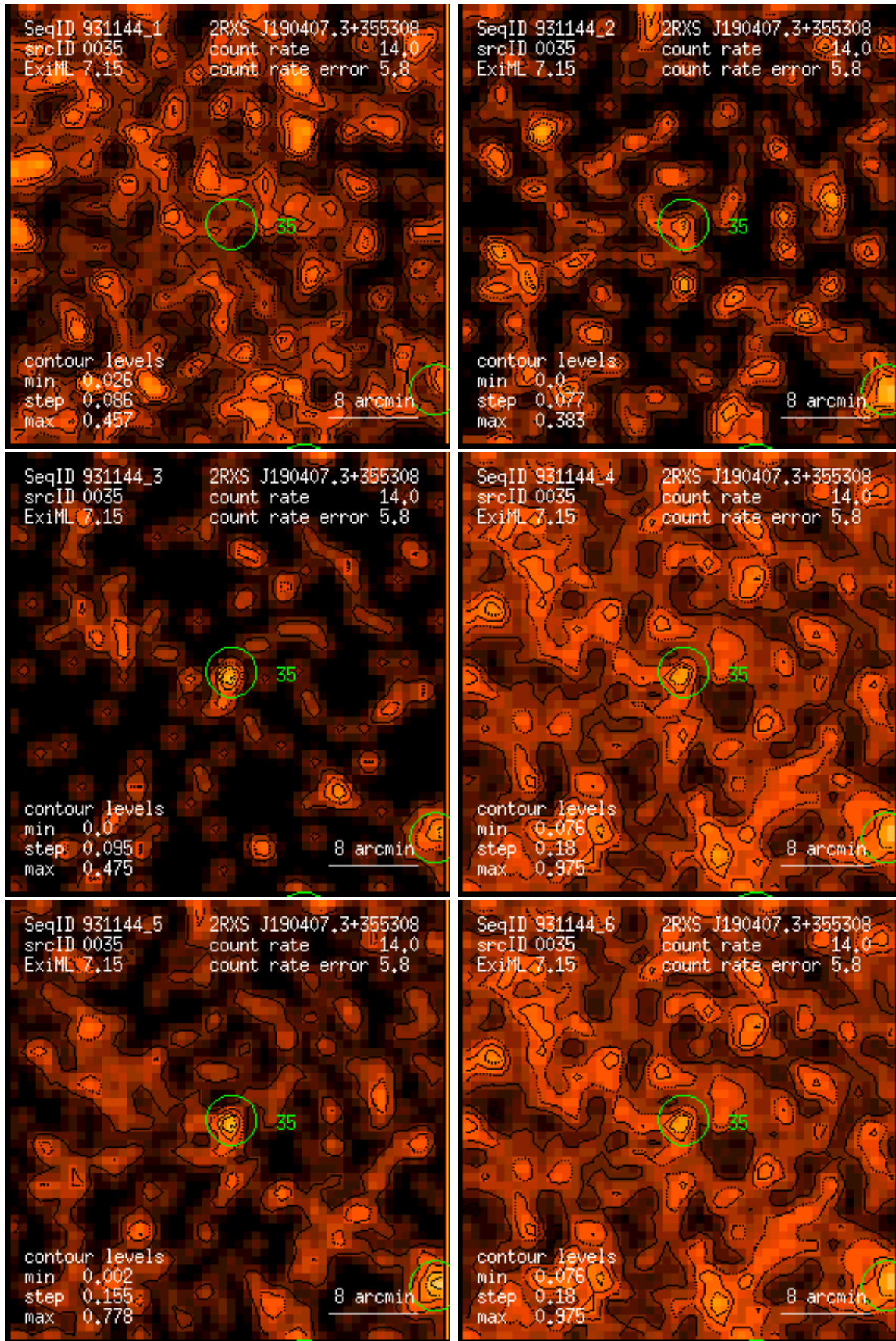
Figure 35: RASS 931144: detection 0035: band rate images, Gaussian filter: (1) PSPC channels 11 – 41, (2) 52 – 90, (3) 91 – 201, (4) 11 – 235, (5) 52 – 201, (6) 11 – 201. Broad band rates in counts/ks. Band rate contour levels in counts/ks/arcmin 2 .
