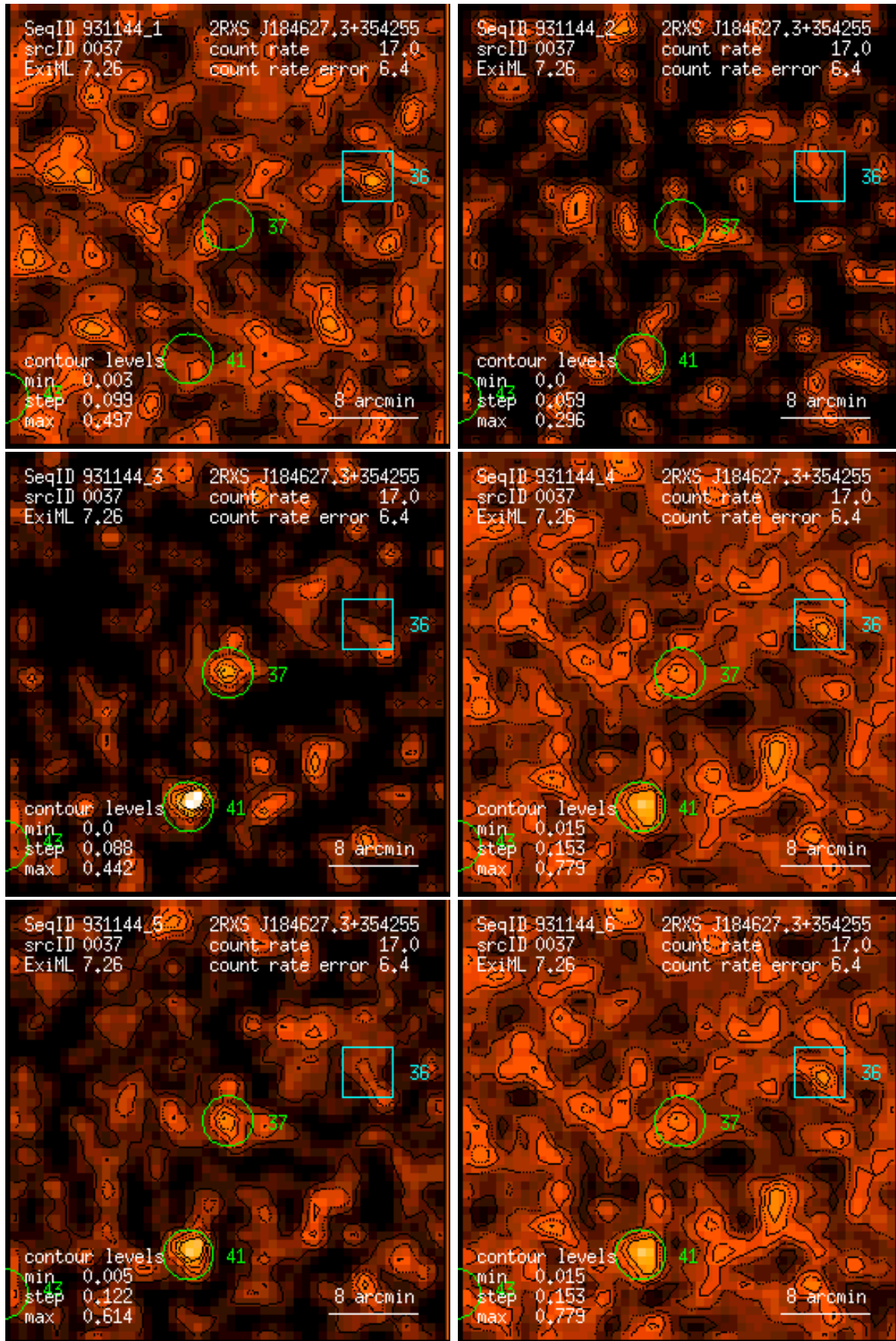
Figure 37: RASS 931144: detection 0037: band rate images, Gaussian filter: (1) PSPC channels 11 – 41, (2) 52 – 90, (3) 91 – 201, (4) 11 – 235, (5) 52 – 201, (6) 11 – 201. Broad band rates in counts/ks. Band rate contour levels in counts/ks/arcmin 2 .
