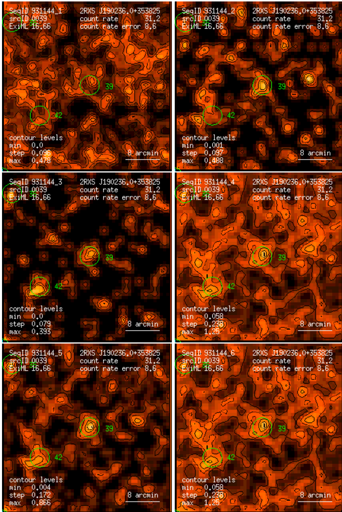
Figure 39: RASS 931144: detection 0039: band rate images, Gaussian filter: (1) PSPC channels 11 – 41, (2) 52 – 90, (3) 91 – 201, (4) 11 – 235, (5) 52 – 201, (6) 11 – 201. Broad band rates in counts/ks. Band rate contour levels in counts/ks/arcmin 2 .
