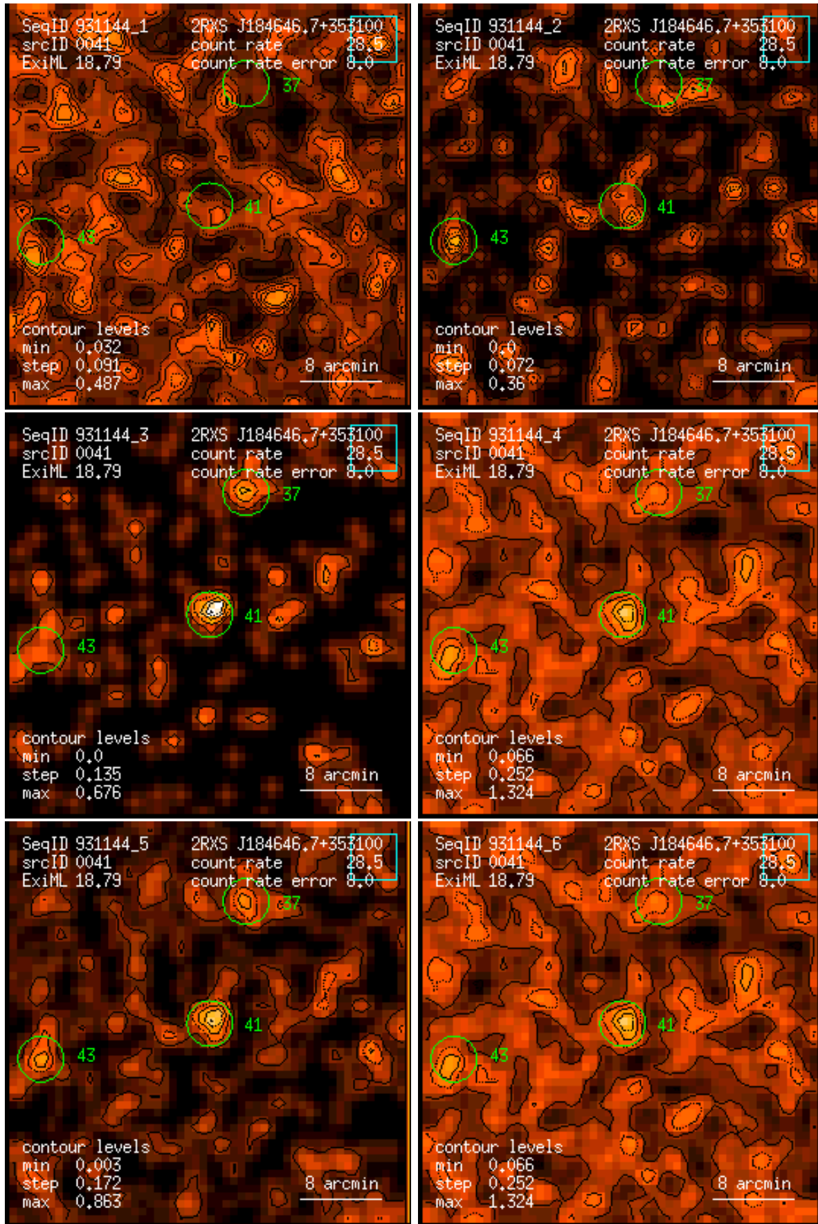
Figure 41: RASS 931144: detection 0041: band rate images, Gaussian filter: (1) PSPC channels 11 – 41, (2) 52 – 90, (3) 91 – 201, (4) 11 – 235, (5) 52 – 201, (6) 11 – 201. Broad band rates in counts/ks. Band rate contour levels in counts/ks/arcmin 2 .
