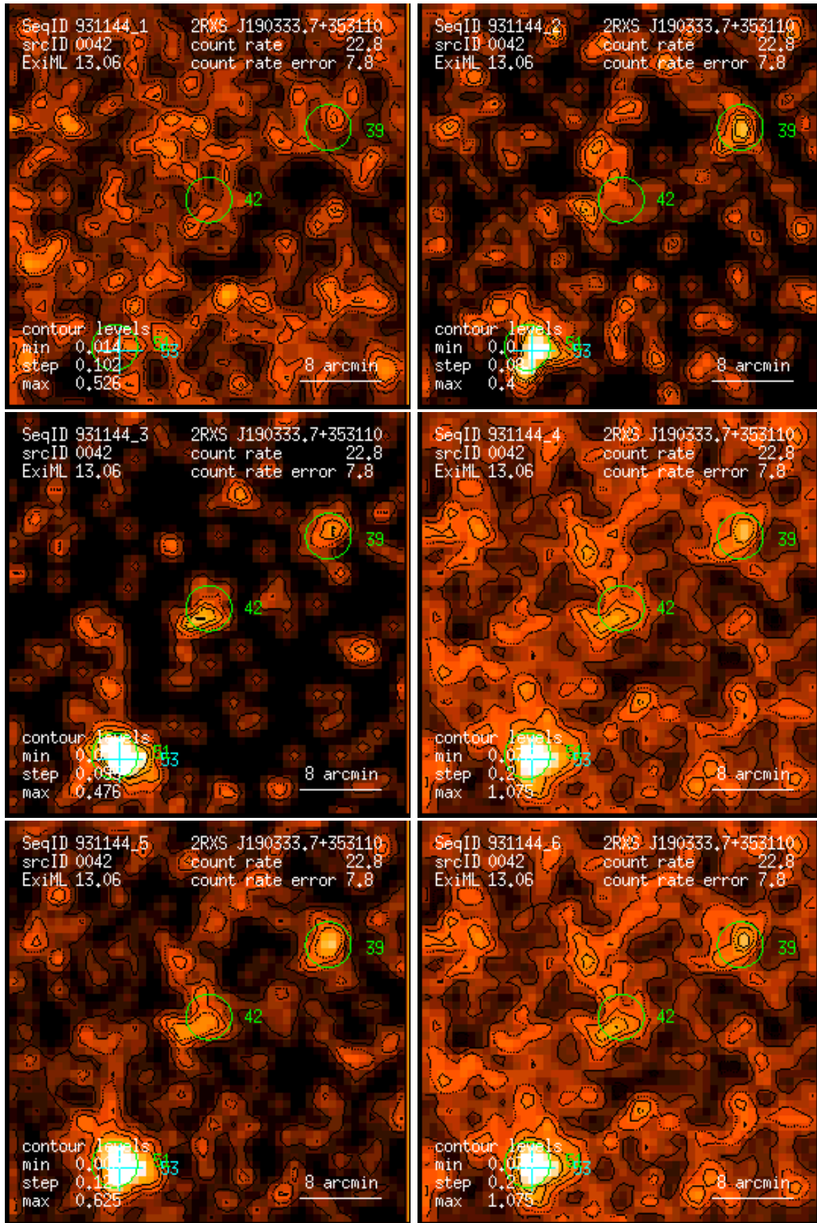
Figure 42: RASS 931144: detection 0042: band rate images, Gaussian filter: (1) PSPC channels 11 – 41, (2) 52 – 90, (3) 91 – 201, (4) 11 – 235, (5) 52 – 201, (6) 11 – 201. Broad band rates in counts/ks. Band rate contour levels in counts/ks/arcmin 2 .
