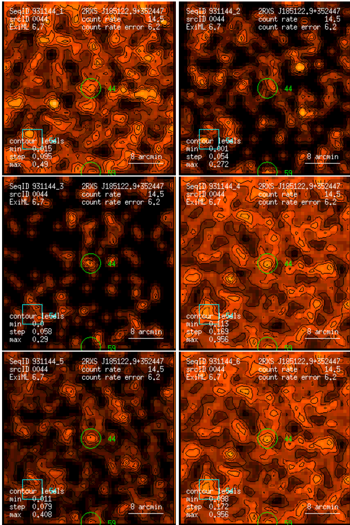
Figure 44: RASS 931144: detection 0044: band rate images, Gaussian filter: (1) PSPC channels 11 – 41, (2) 52 – 90, (3) 91 – 201, (4) 11 – 235, (5) 52 – 201, (6) 11 – 201. Broad band rates in counts/ks. Band rate contour levels in counts/ks/arcmin 2 .
