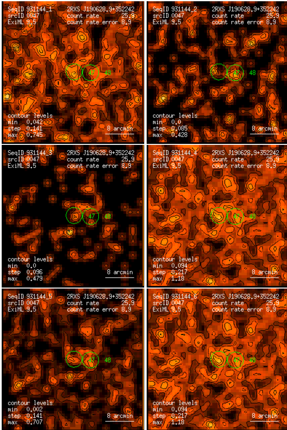
Figure 47: RASS 931144: detection 0047: band rate images, Gaussian filter: (1) PSPC channels 11 – 41, (2) 52 – 90, (3) 91 – 201, (4) 11 – 235, (5) 52 – 201, (6) 11 – 201. Broad band rates in counts/ks. Band rate contour levels in counts/ks/arcmin 2 .
