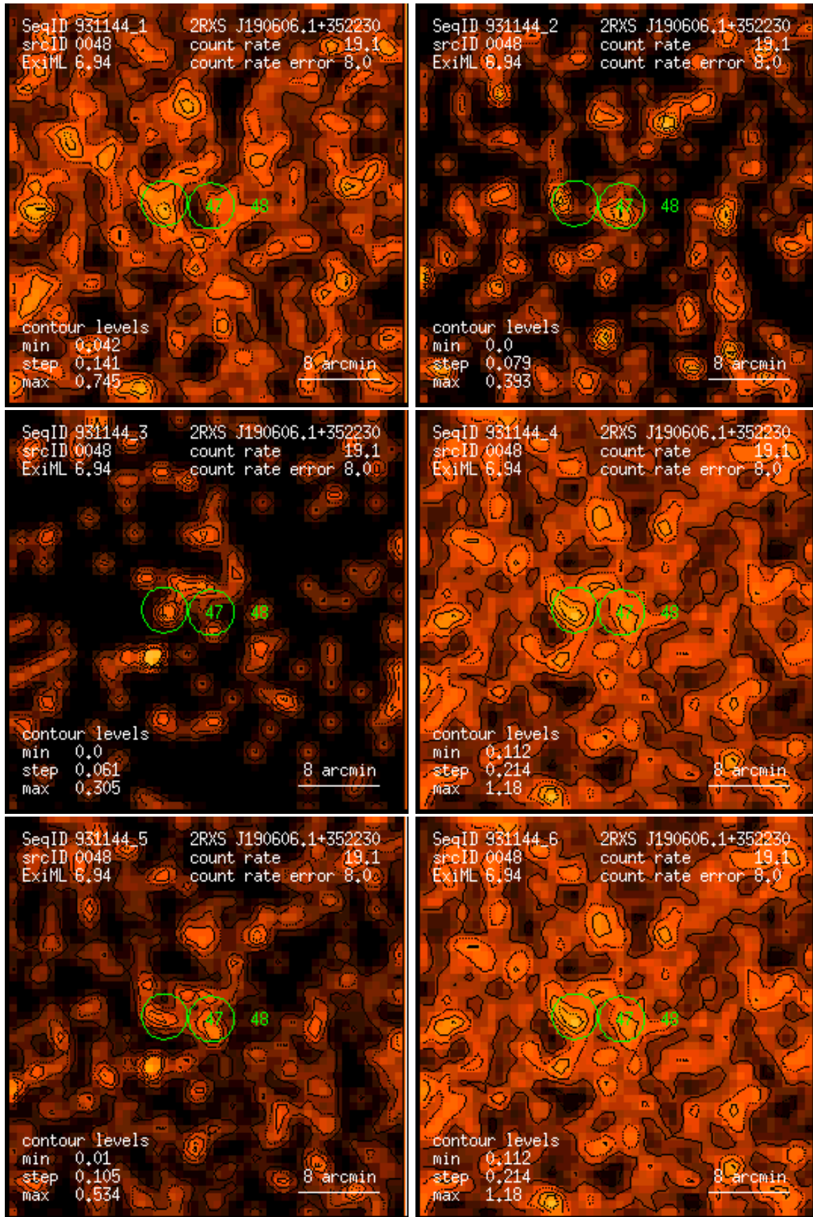
Figure 48: RASS 931144: detection 0048: band rate images, Gaussian filter: (1) PSPC channels 11 – 41, (2) 52 – 90, (3) 91 – 201, (4) 11 – 235, (5) 52 – 201, (6) 11 – 201. Broad band rates in counts/ks. Band rate contour levels in counts/ks/arcmin 2 .
