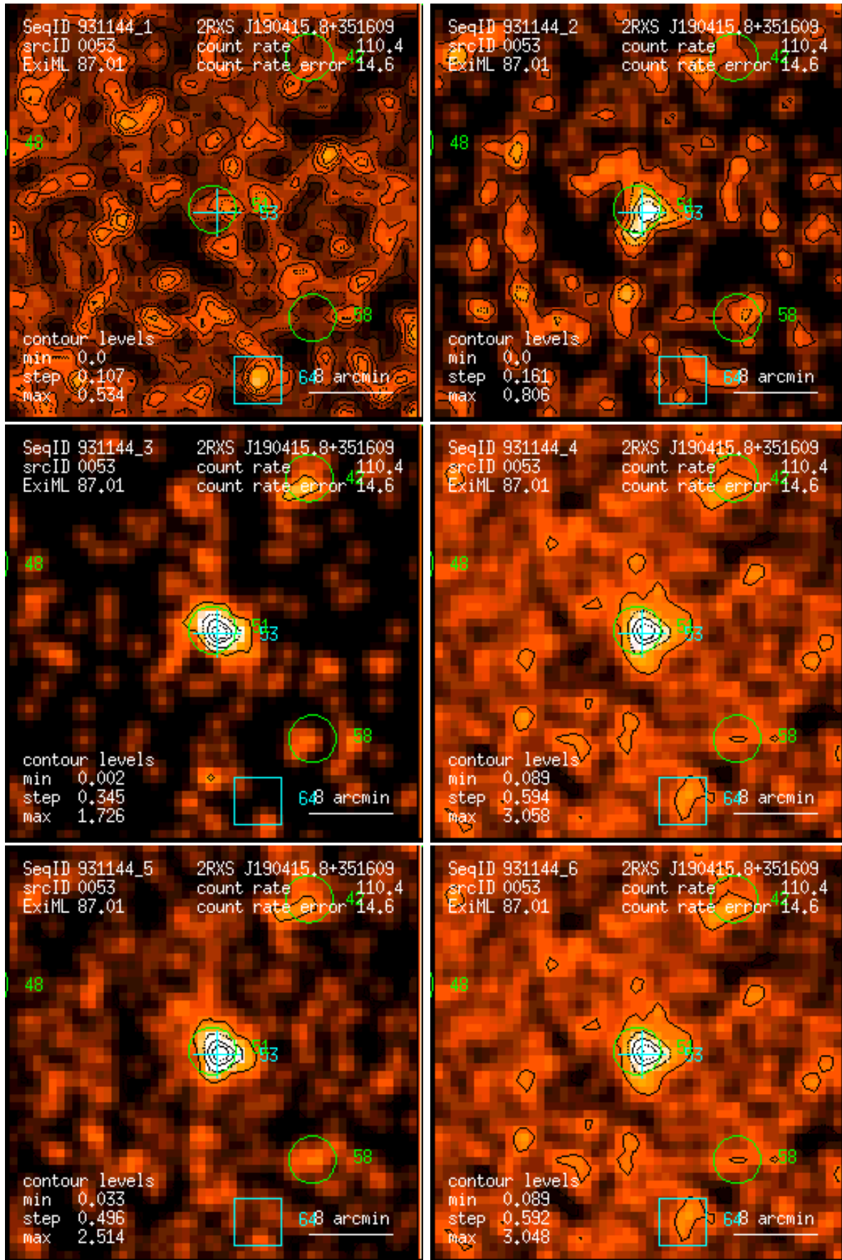
Figure 53: RASS 931144: detection 0053: band rate images, Gaussian filter: (1) PSPC channels 11 – 41, (2) 52 – 90, (3) 91 – 201, (4) 11 – 235, (5) 52 – 201, (6) 11 – 201. Broad band rates in counts/ks. Band rate contour levels in counts/ks/arcmin 2 .
