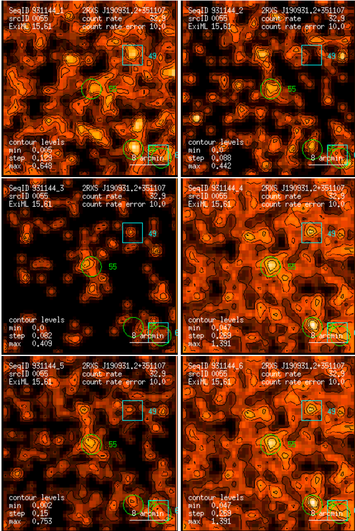
Figure 55: RASS 931144: detection 0055: band rate images, Gaussian filter: (1) PSPC channels 11 – 41, (2) 52 – 90, (3) 91 – 201, (4) 11 – 235, (5) 52 – 201, (6) 11 – 201. Broad band rates in counts/ks. Band rate contour levels in counts/ks/arcmin 2 .
