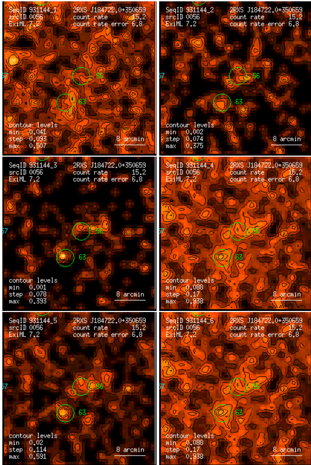
Figure 56: RASS 931144: detection 0056: band rate images, Gaussian filter: (1) PSPC channels 11 – 41, (2) 52 – 90, (3) 91 – 201, (4) 11 – 235, (5) 52 – 201, (6) 11 – 201. Broad band rates in counts/ks. Band rate contour levels in counts/ks/arcmin 2 .
