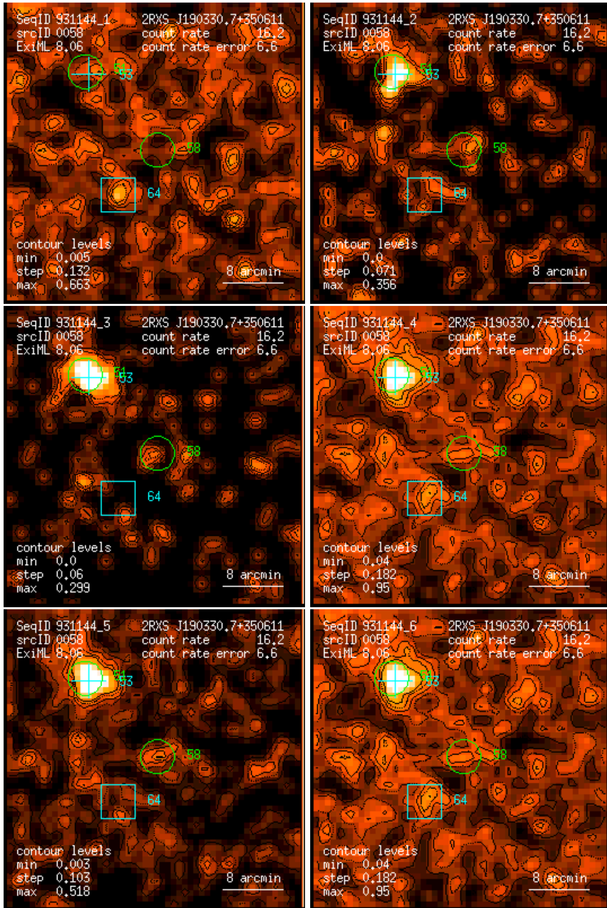
Figure 58: RASS 931144: detection 0058: band rate images, Gaussian filter: (1) PSPC channels 11 – 41, (2) 52 – 90, (3) 91 – 201, (4) 11 – 235, (5) 52 – 201, (6) 11 – 201. Broad band rates in counts/ks. Band rate contour levels in counts/ks/arcmin 2 .
