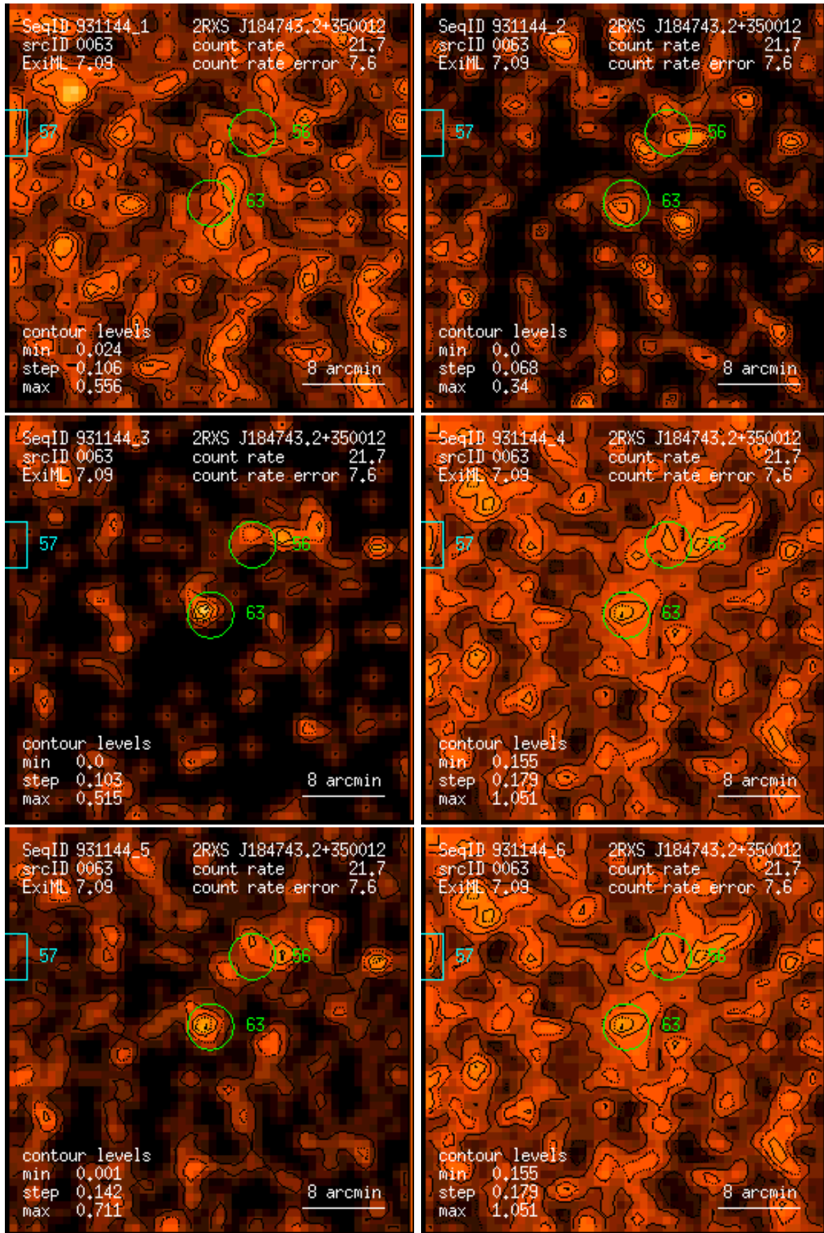
Figure 63: RASS 931144: detection 0063: band rate images, Gaussian filter: (1) PSPC channels 11 – 41, (2) 52 – 90, (3) 91 – 201, (4) 11 – 235, (5) 52 – 201, (6) 11 – 201. Broad band rates in counts/ks. Band rate contour levels in counts/ks/arcmin 2 .
