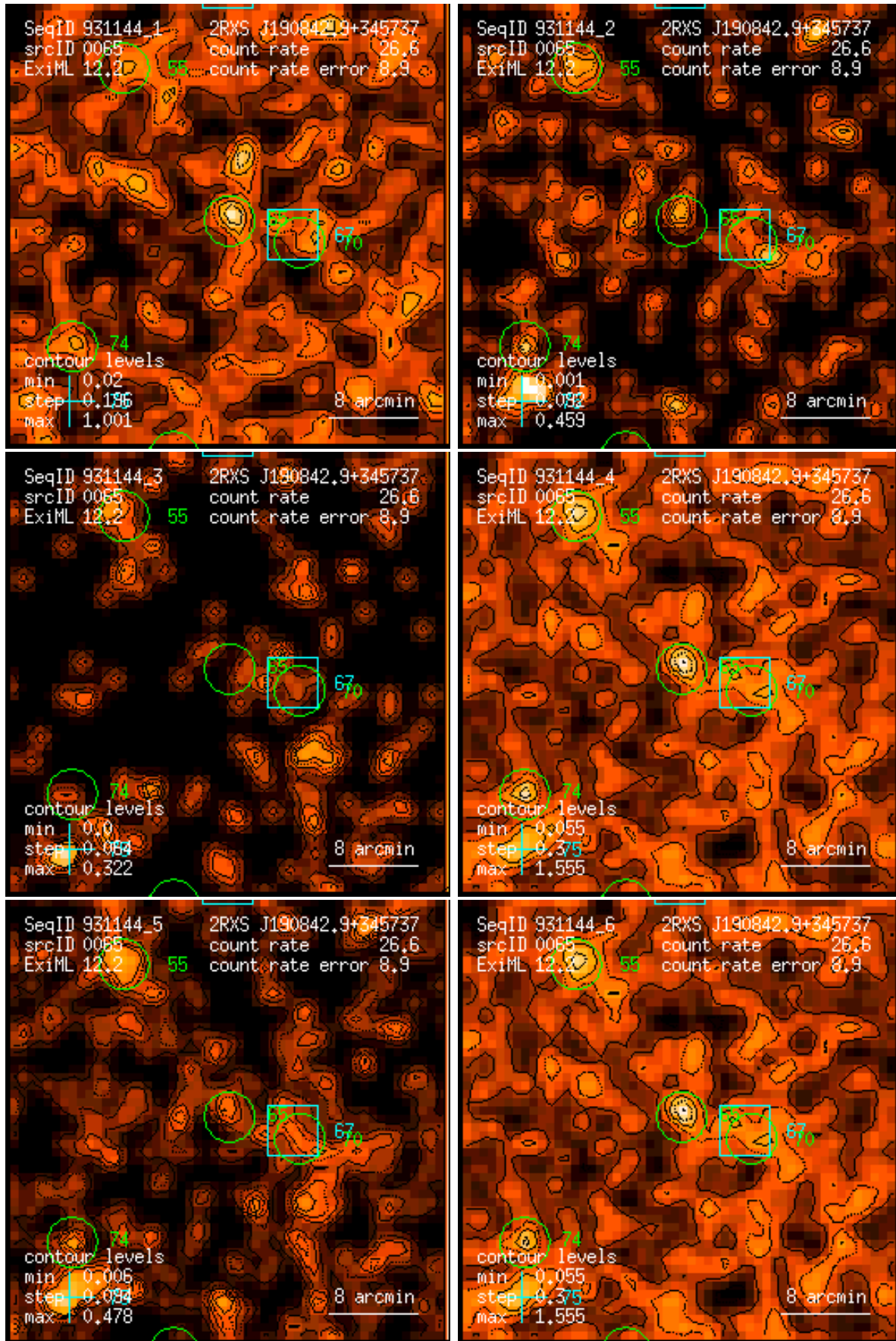
Figure 65: RASS 931144: detection 0065: band rate images, Gaussian filter: (1) PSPC channels 11 – 41, (2) 52 – 90, (3) 91 – 201, (4) 11 – 235, (5) 52 – 201, (6) 11 – 201. Broad band rates in counts/ks. Band rate contour levels in counts/ks/arcmin 2 .
