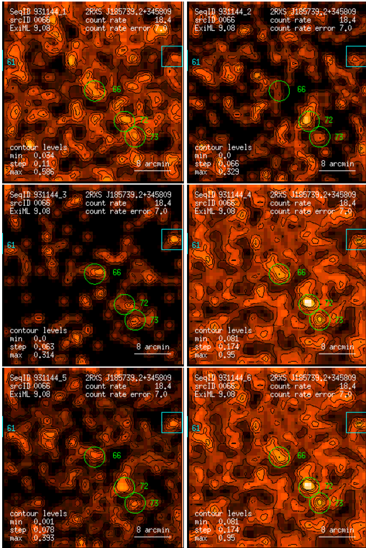
Figure 66: RASS 931144: detection 0066: band rate images, Gaussian filter: (1) PSPC channels 11 – 41, (2) 52 – 90, (3) 91 – 201, (4) 11 – 235, (5) 52 – 201, (6) 11 – 201. Broad band rates in counts/ks. Band rate contour levels in counts/ks/arcmin 2 .
