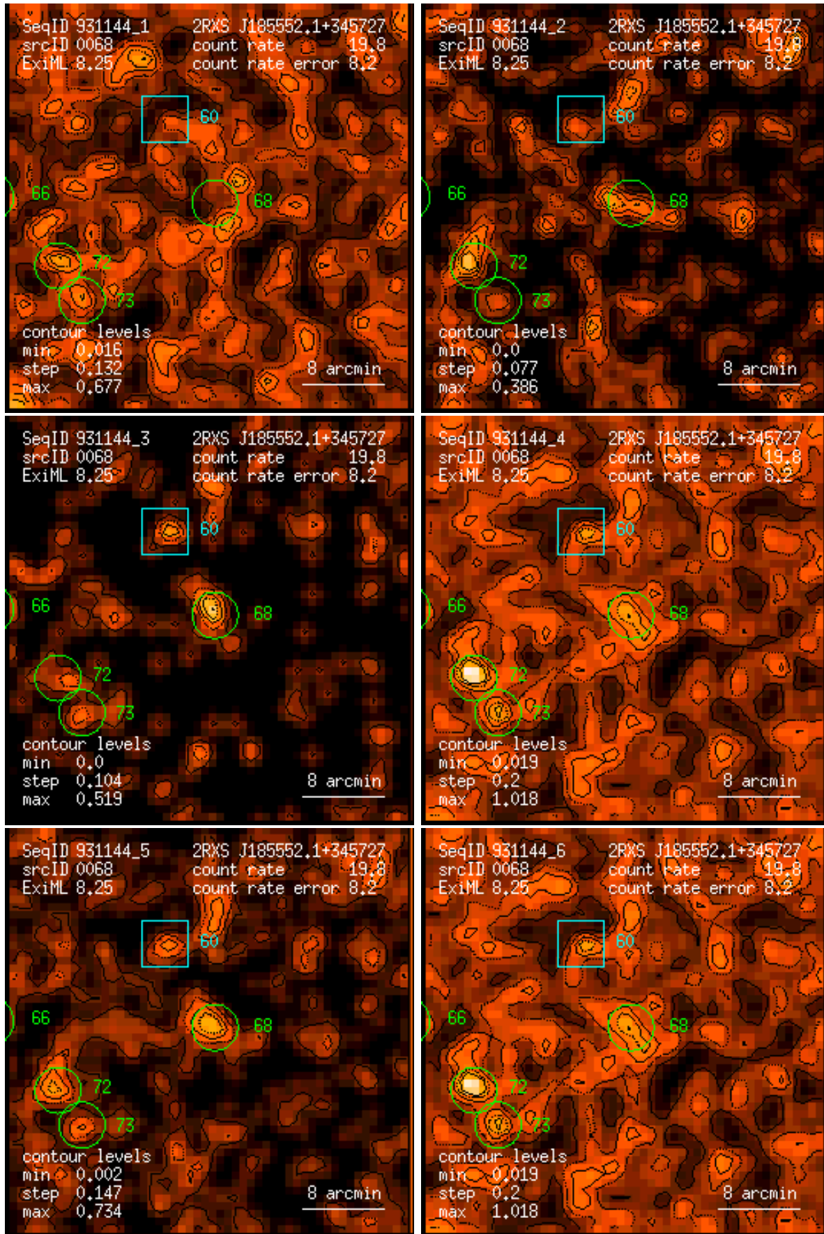
Figure 68: RASS 931144: detection 0068: band rate images, Gaussian filter: (1) PSPC channels 11 – 41, (2) 52 – 90, (3) 91 – 201, (4) 11 – 235, (5) 52 – 201, (6) 11 – 201. Broad band rates in counts/ks. Band rate contour levels in counts/ks/arcmin 2 .
