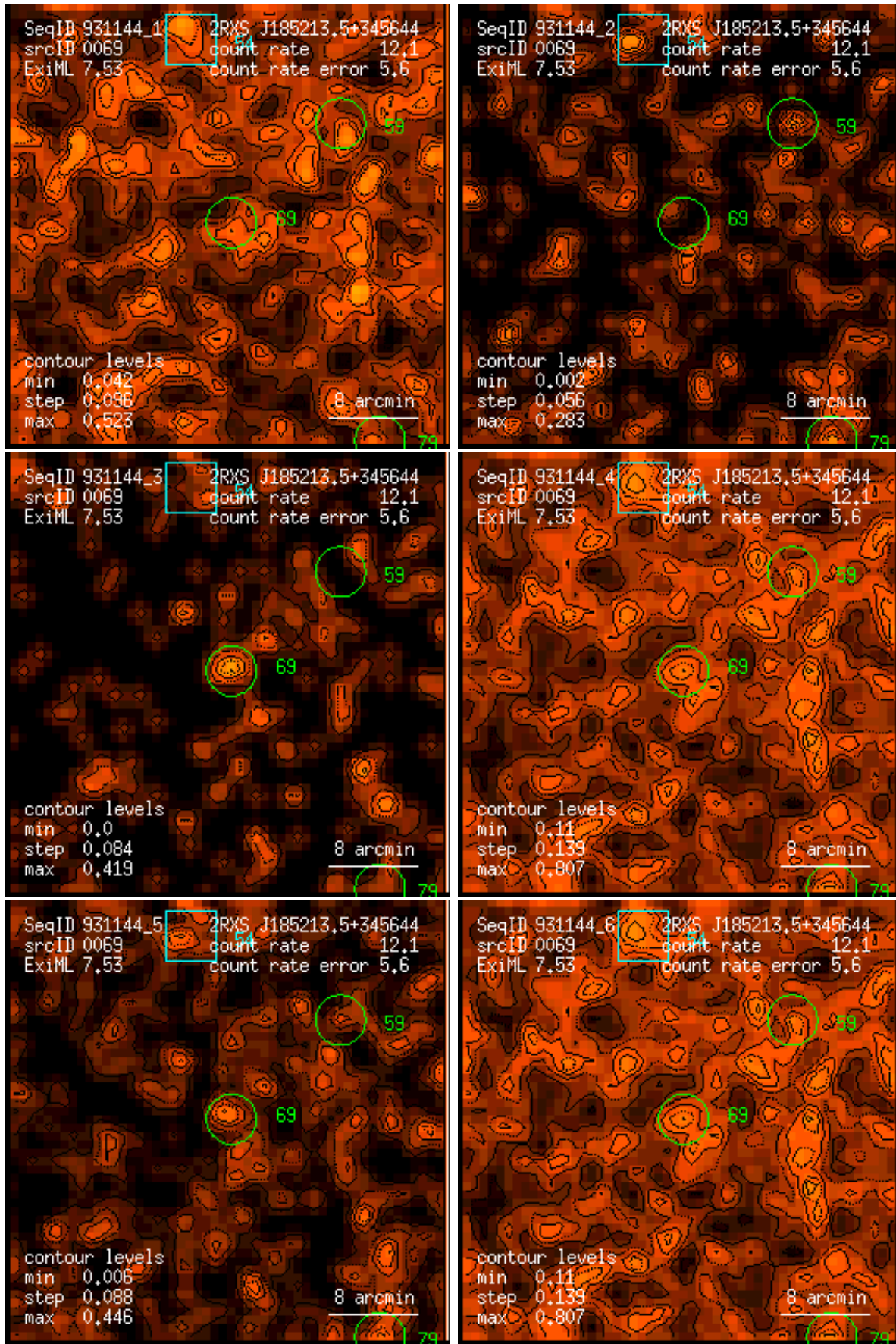
Figure 69: RASS 931144: detection 0069: band rate images, Gaussian filter: (1) PSPC channels 11 – 41, (2) 52 – 90, (3) 91 – 201, (4) 11 – 235, (5) 52 – 201, (6) 11 – 201. Broad band rates in counts/ks. Band rate contour levels in counts/ks/arcmin 2 .
