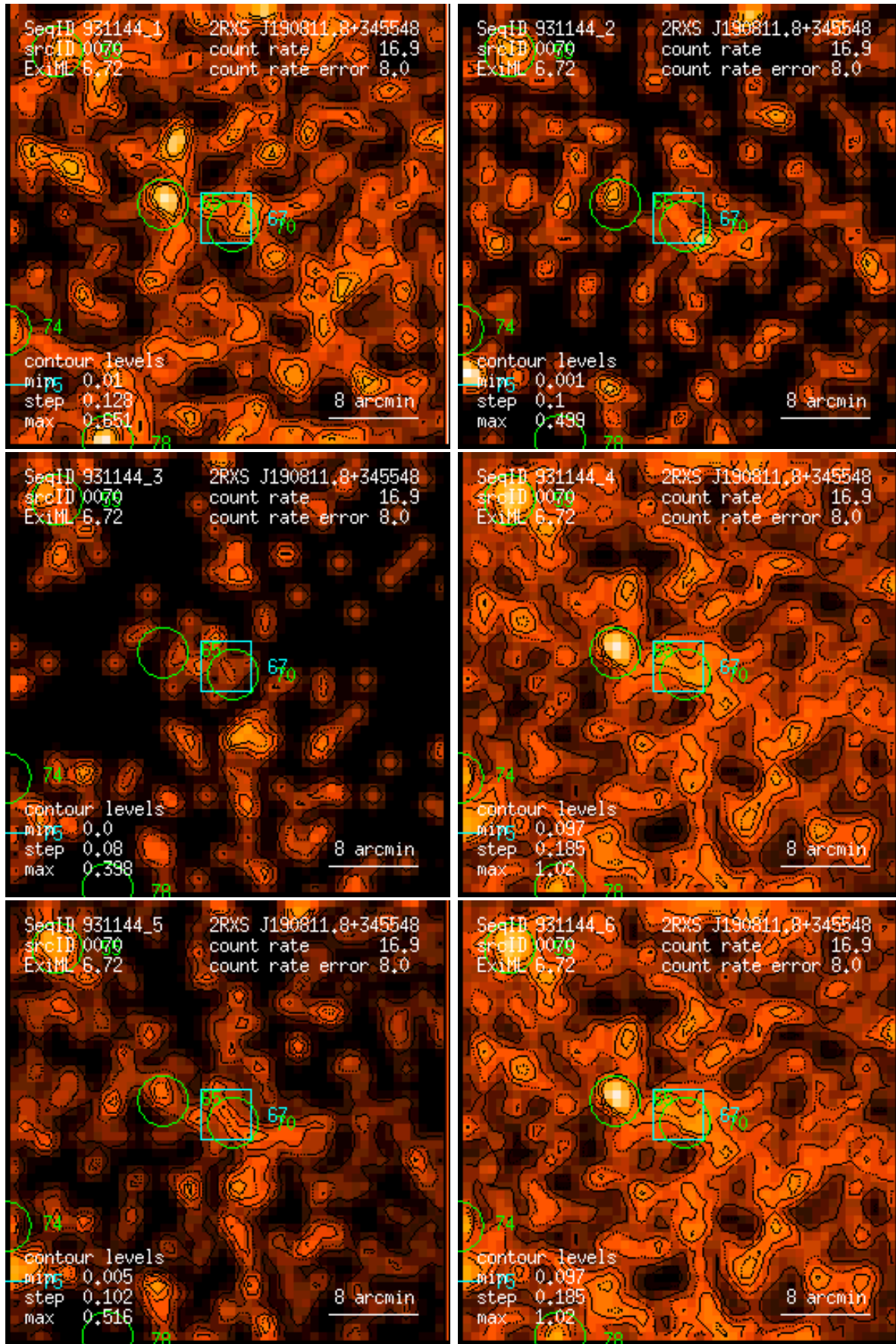
Figure 70: RASS 931144: detection 0070: band rate images, Gaussian filter: (1) PSPC channels 11 – 41, (2) 52 – 90, (3) 91 – 201, (4) 11 – 235, (5) 52 – 201, (6) 11 – 201. Broad band rates in counts/ks. Band rate contour levels in counts/ks/arcmin 2 .
