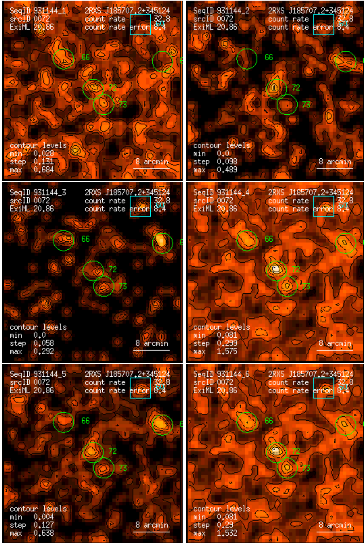
Figure 72: RASS 931144: detection 0072: band rate images, Gaussian filter: (1) PSPC channels 11 – 41, (2) 52 – 90, (3) 91 – 201, (4) 11 – 235, (5) 52 – 201, (6) 11 – 201. Broad band rates in counts/ks. Band rate contour levels in counts/ks/arcmin 2 .
