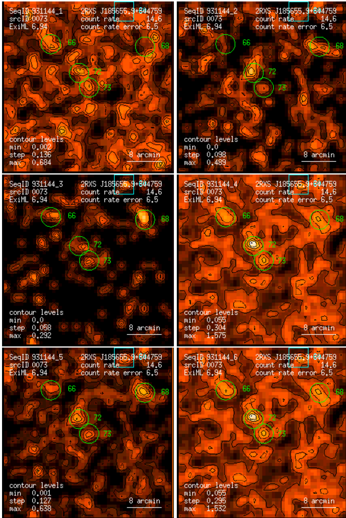
Figure 73: RASS 931144: detection 0073: band rate images, Gaussian filter: (1) PSPC channels 11 – 41, (2) 52 – 90, (3) 91 – 201, (4) 11 – 235, (5) 52 – 201, (6) 11 – 201. Broad band rates in counts/ks. Band rate contour levels in counts/ks/arcmin 2 .
