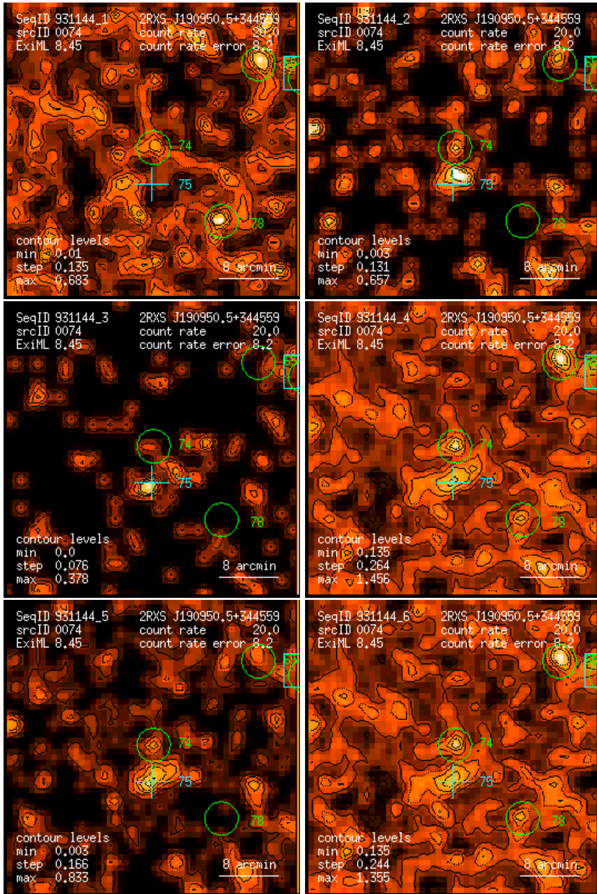
Figure 74: RASS 931144: detection 0074: band rate images, Gaussian filter: (1) PSPC channels 11 – 41, (2) 52 – 90, (3) 91 – 201, (4) 11 – 235, (5) 52 – 201, (6) 11 – 201. Broad band rates in counts/ks. Band rate contour levels in counts/ks/arcmin 2 .
